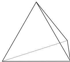
Figure 3: The three simplex, \Delta^3 . Note: This is not the standard embedding in \mathbb{R}^4 !
