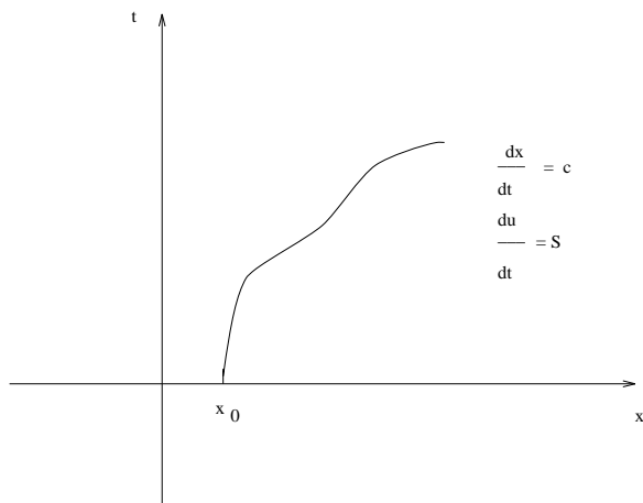
Figure 12: u(x_0, 0) = f(x_0)
