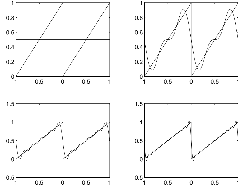
Figure 31: Graph of f(x) given by example 4 ( L = 1 ) and the N^{\text{th}} partial sums for N = 1, 5, 10, 20 . Notice that for L = 1 all cosine terms and odd sine terms vanish, thus the first term is the constant .5
