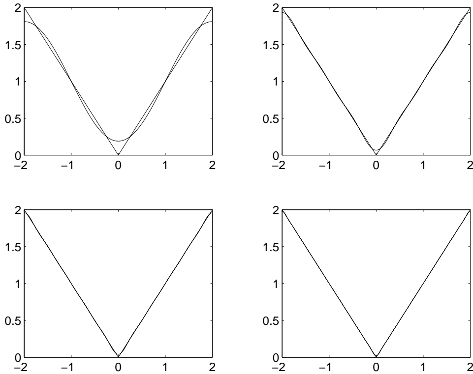
Figure 40: Graph of f(x) = |x| and the N^{\text{th}} partial sums for N = 1, 5, 10, 20
