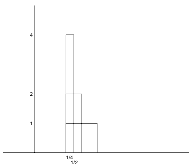
Figure 61: Several impulses of unit area
