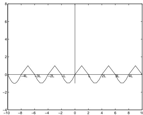
Figure 38: Sketch of the periodic extension
