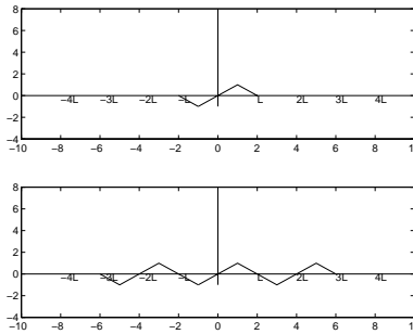
Figure 42: Sketch of the Fourier sine series and the periodic odd extension
