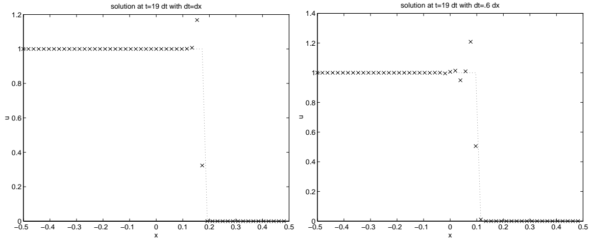
Figure 85: Solution of Burgers' equation using Lax Wendroff method
