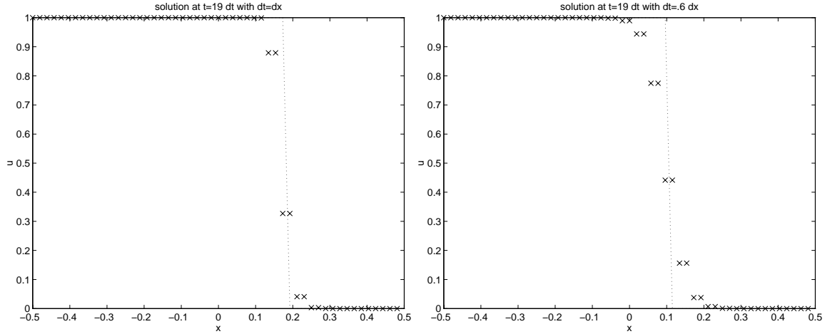
Figure 84: Solution of Burgers' equation using Lax method
