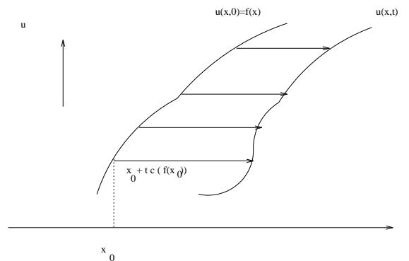
Figure 13: Graphical solution
