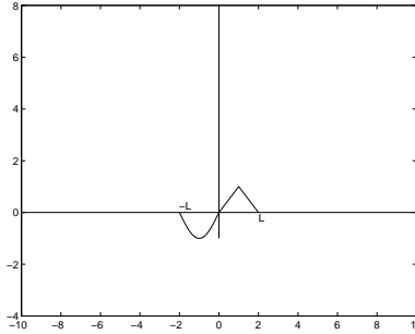
Figure 41: Sketch of f(x) given in Example 10
