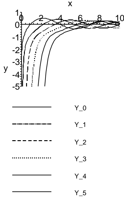
Figure 50: Bessel functions Y_n, n = 0, \dots, 5
