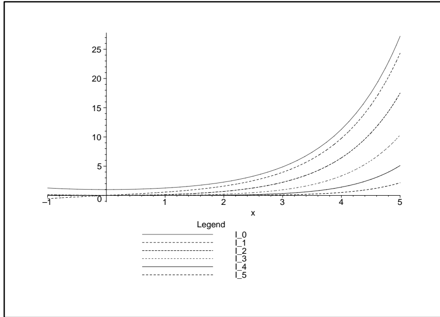
Figure 51: Bessel functions I_n, n = 0, \dots, 4
