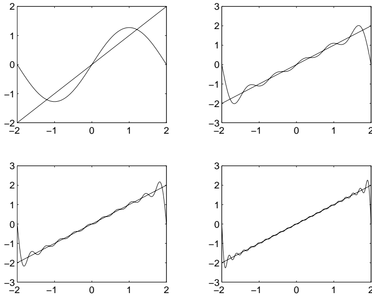
Figure 28: Graph of f(x) = x and the N^{\text{th}} partial sums for N = 1, 5, 10, 20
