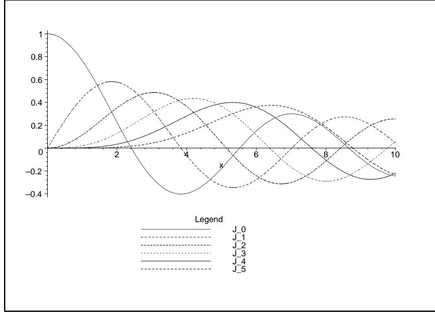
Figure 49: Bessel functions J_n, n = 0, \dots, 5
