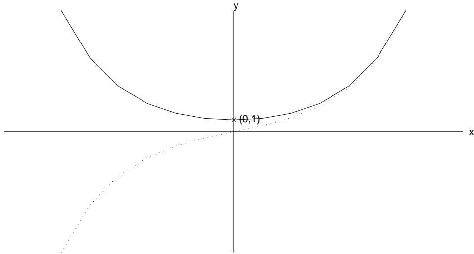
Figure 27: \sinh x and \cosh x
