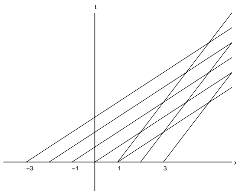
Figure 16: Intersecting characteristics
