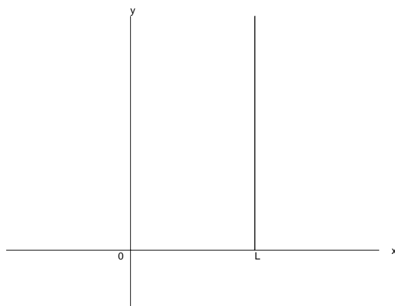
Figure 59: Domain for Laplace's equation example
