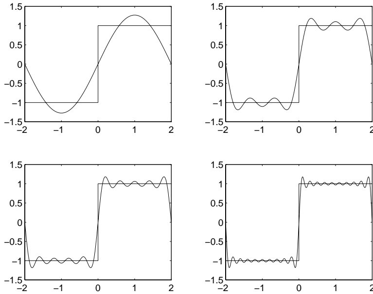
Figure 29: Graph of f(x) given in Example 3 and the N^{\text{th}} partial sums for N = 1, 5, 10, 20
