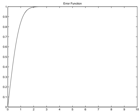
Figure 58: Plot of the error function erf(x)
