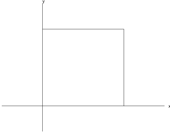
Figure 55: Rectangular domain
