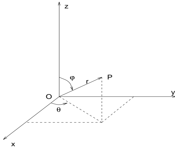
Figure 3.4: Spherical coordinates.
