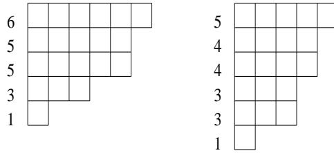
Figure 7.4: The conjugate of (6,5,5,3,1) is (5,4,4,3,3,1)
