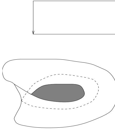
Figure 3.2: The Mobius band.
