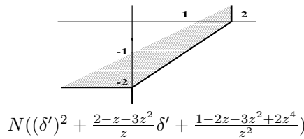
Figure 3.6: Newton Polygons for Example 3.53
