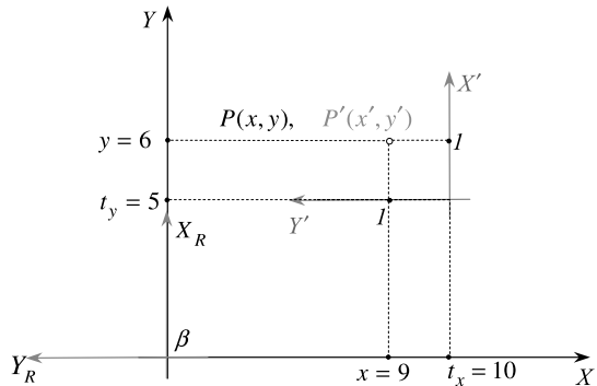
Fig. 8.5 The X'Y' axial system is translated (10, 5) and rotated 90^\circ
