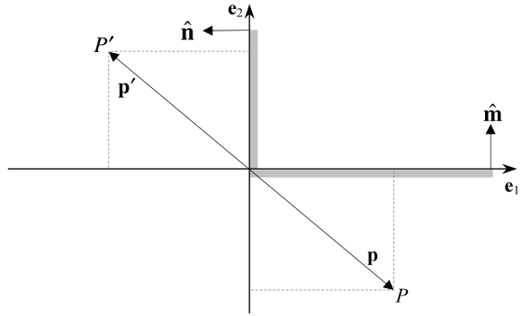
Fig. 12.5 Rotating a point by 180°
