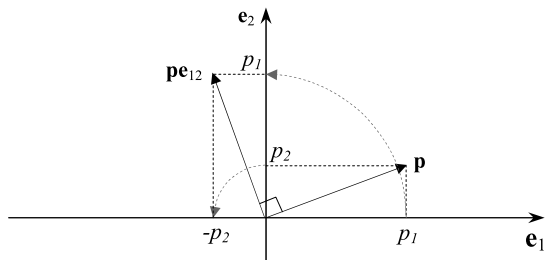
Fig. 7.4 \mathbf{p}\mathbf{e}_{12} rotates \mathbf{p} , 90^\circ
