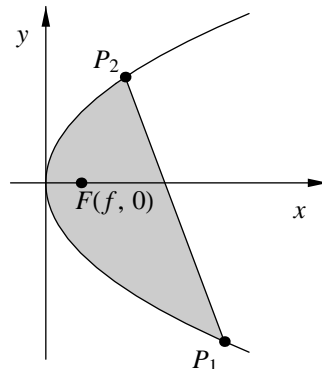
Figure 17.8: Area of a parabolic segment.
