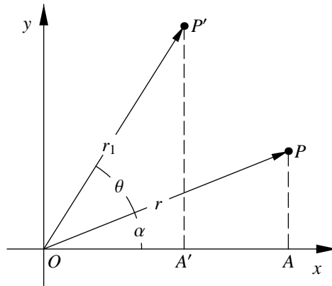
Figure 15.1: Rotation transformation.
