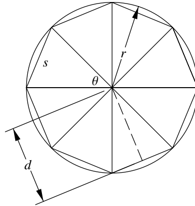
Figure 16.1: Circle approximated by an inscribed polygon.
