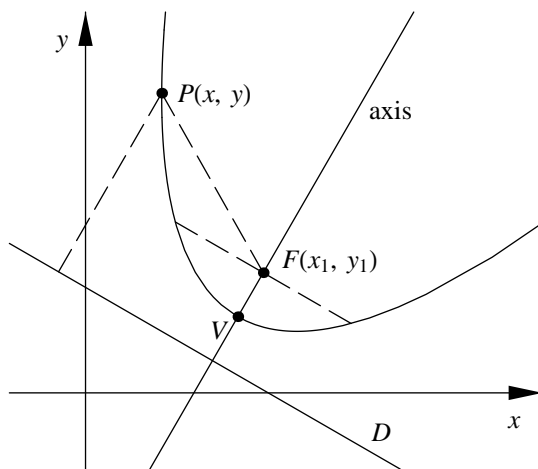
Figure 9.1: Definition of a parabola.
