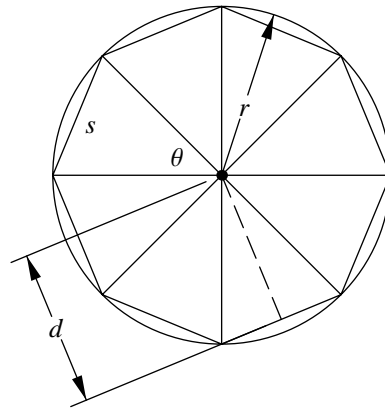
Figure 17.4: Circle approximated by an inscribed polygon.
