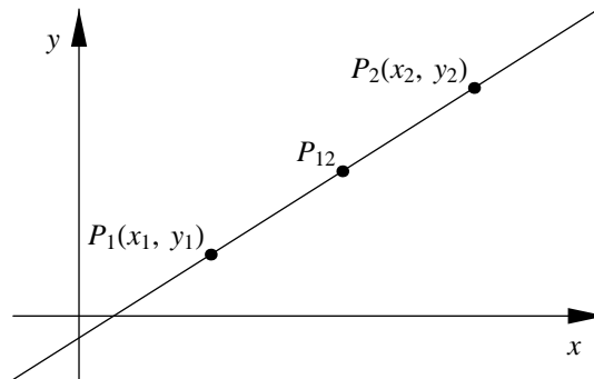
Figure 3.4: Midpoint between two points.
