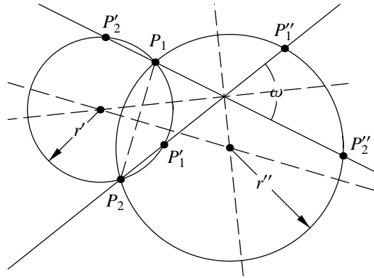
Figure 21.3: Knot circles.
