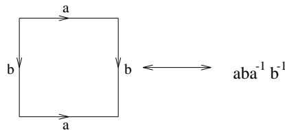
FIGURE 6.1. The torus as an identification space
