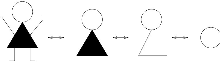
FIGURE 3.5. Homotopy equivalences
