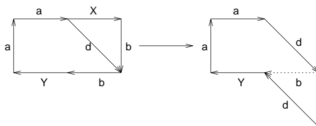
FIGURE 6.21. Assembling crosscaps
