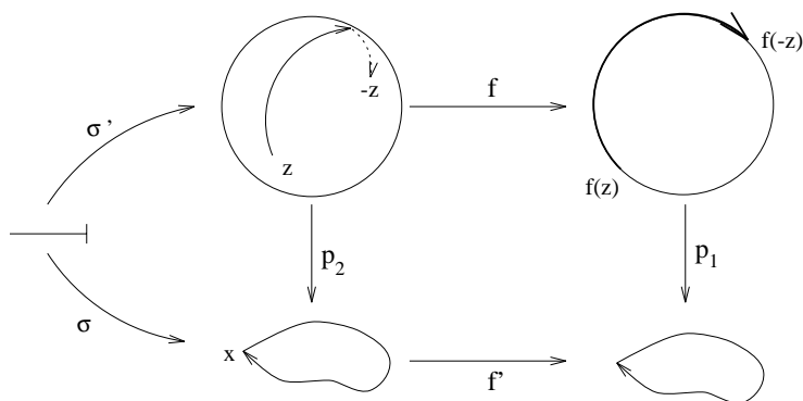
FIGURE 5.7. Borsuk-Ulam Theorem
