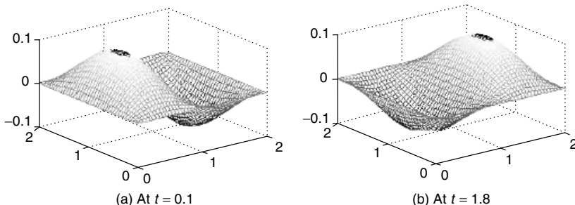
Figure 9.6 The solution of a two-dimensional hyperbolic PDE: vibration of a square membrane (Example 9.5).
