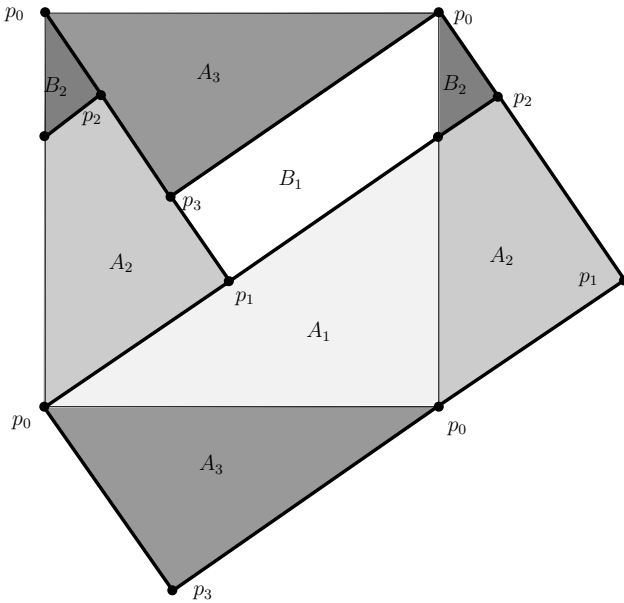
Figure 5.5. Markov partition for the toral automorphism f_M .
