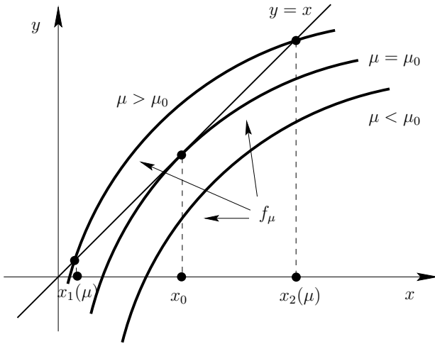
Figure 7.6. Saddle-node bifurcation.
