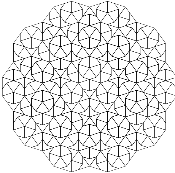
FIGURE 3. A cartwheel patch in a tiling ([246])
