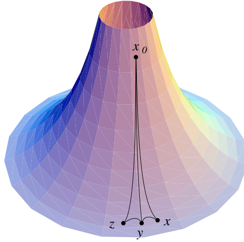
FIGURE 2. Hyperbolic metric space
