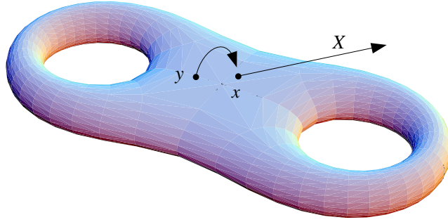
FIGURE 6. The tangent groupoid of M
