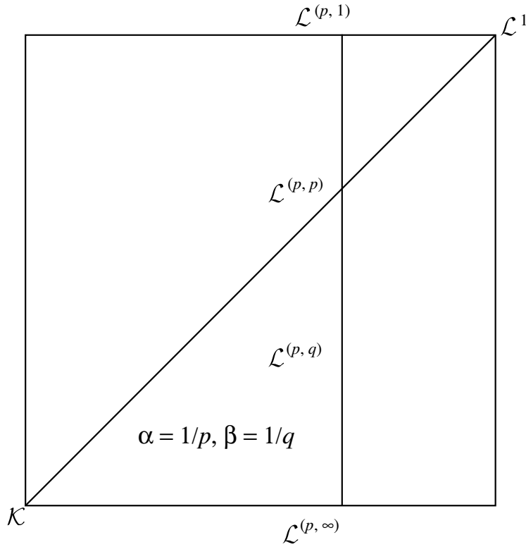
FIGURE 1. Interpolation square
