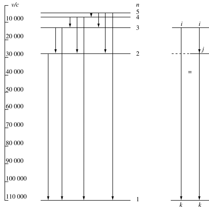
FIGURE 2. The vertical arrows represent the transitions. They are indexed by a pair of indices (i, j) .
