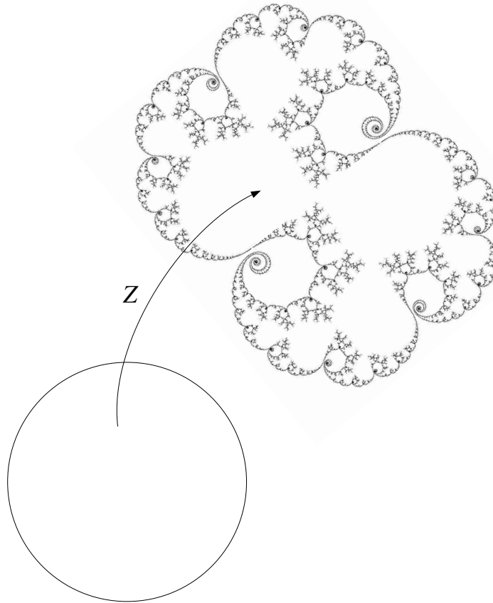
FIGURE 2. Riemann mapping
