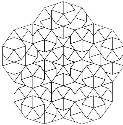
FIGURE 2. A star patch in a tiling ([246])
