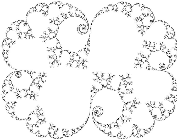
FIGURE 5. A Julia set
