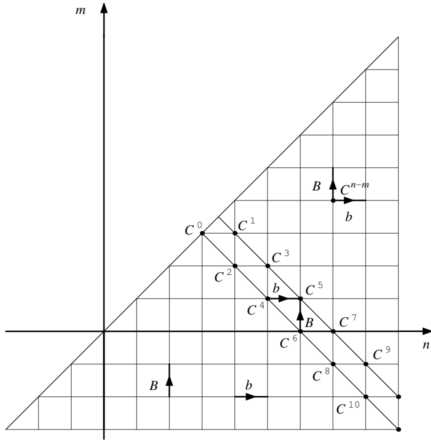
FIGURE 1. The (b, B) bicomplex
