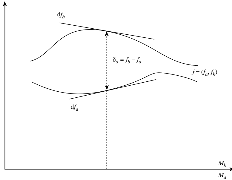
FIGURE 4. Differential of a function on a double-space
