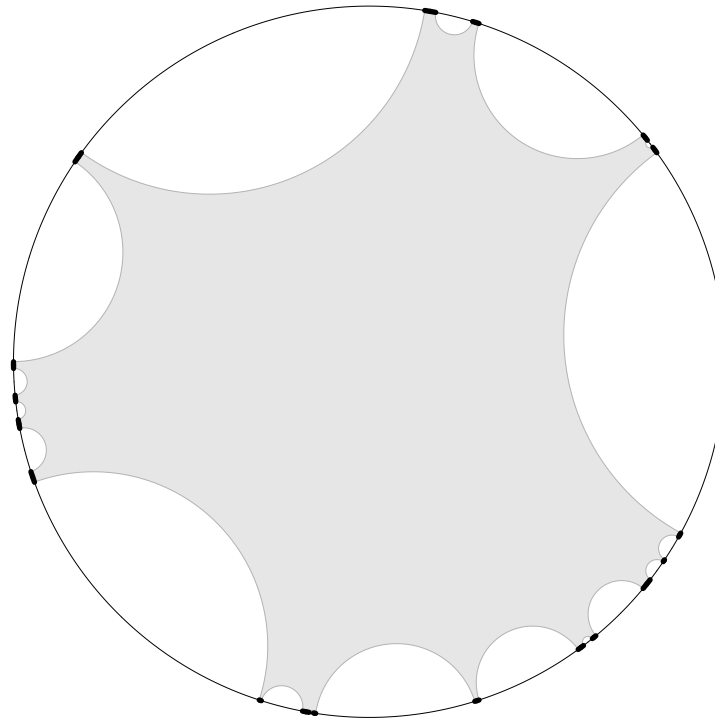
FIGURE 3. Convex hull of a perfect set
