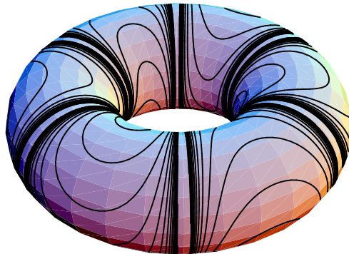
FIGURE 8. Example of type I foliation
