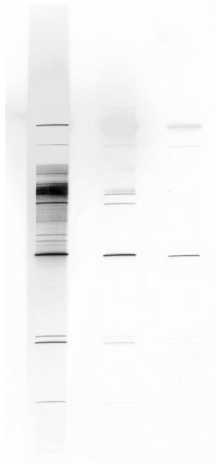
FIGURE 1. Hydrogen Spectrum
