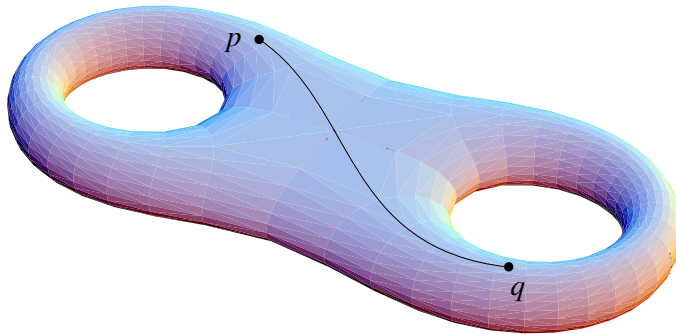
FIGURE 1. Geodesic
