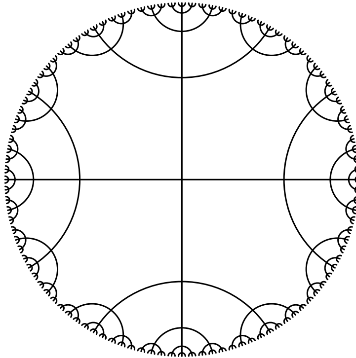
FIGURE 5. Tree
