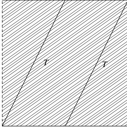
FIGURE 8. The Kronecker foliation with a closed transversal T
