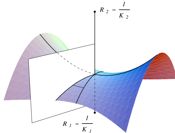
FIGURE 4. Curvature
