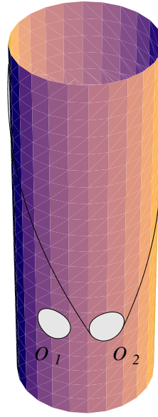
FIGURE 10. Space like regions \mathcal{O}_1 and \mathcal{O}_2 in space-time cylinder
