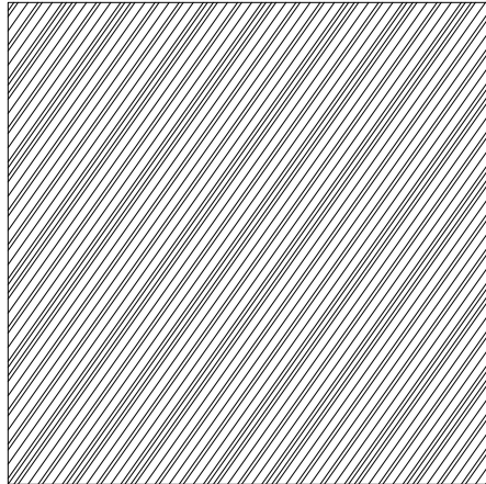
FIGURE 7. Kronecker foliation dy = \sqrt{2} dx
