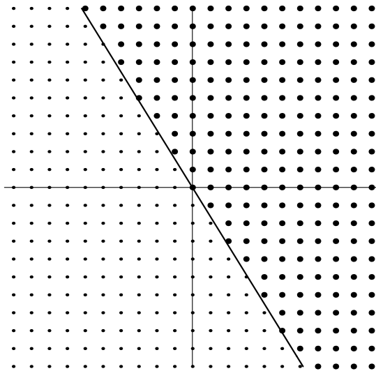
FIGURE 4. K_0^+(A) = \left\{ (n, m) \in \mathbb{Z}^2 ; n \frac{1+\sqrt{5}}{2} + m \geq 0 \right\}
