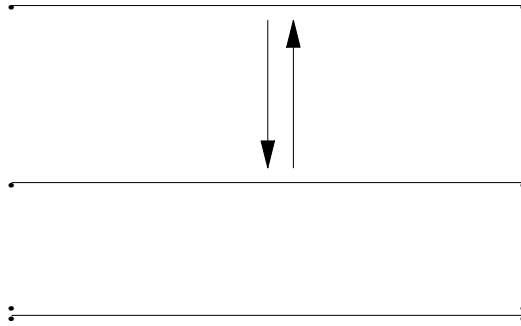
FIGURE 2. The dual of the infinite dihedral group. The points inside the intervals are identified, but not the endpoints.
