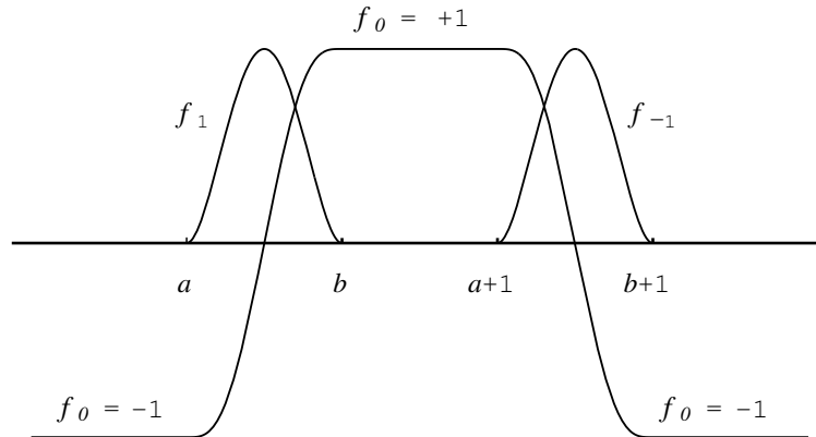
FIGURE 6. Powers-Rieffel Idempotent
