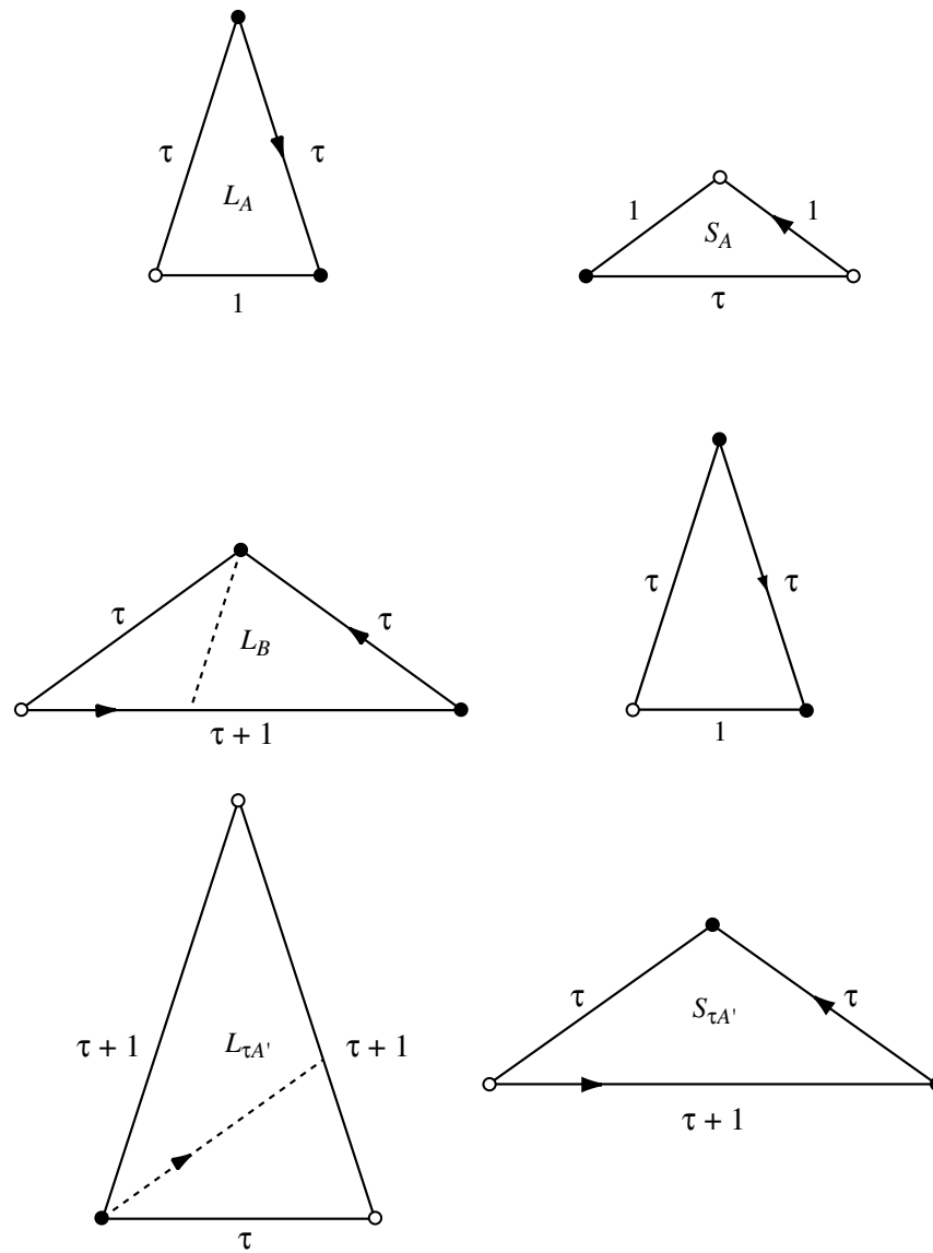
FIGURE 10. Elementary tiles (see [246])
