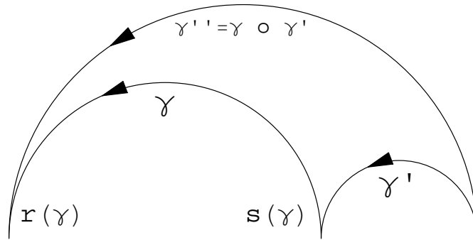
FIGURE 5. Groupoid.
