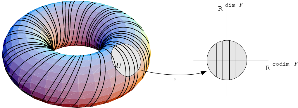
FIGURE 6. Foliation
