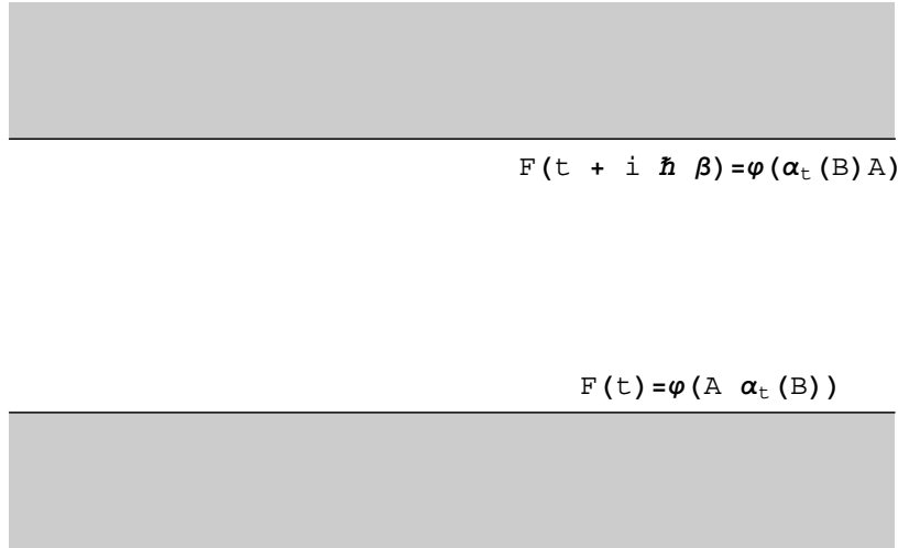
FIGURE 3. The KMS condition
