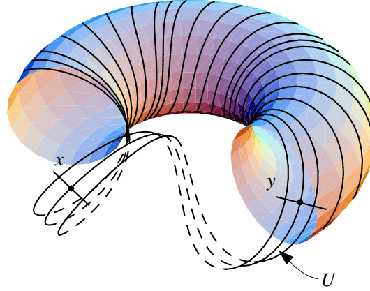
FIGURE 9. x and y belong to the same leaf, U is a domain of foliation chart containing x, y and x, y belong to the same plaque.
