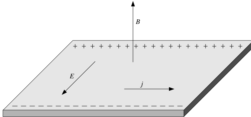
FIGURE 7. Hall current
