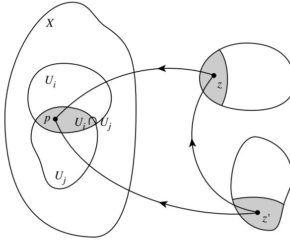
FIGURE 1. One identifies z with z' using the algebra of matrices.
