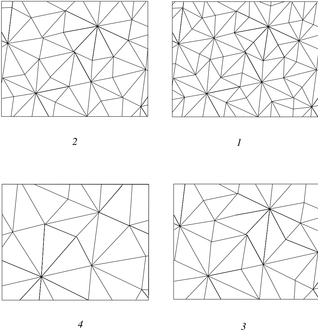
FIGURE 11. A sequence of triangulation patches (see [246])
