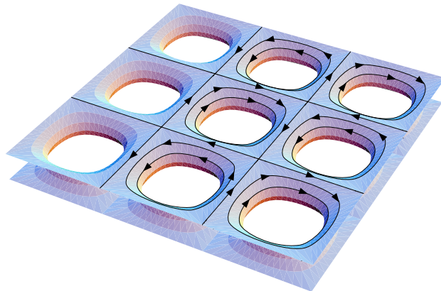
FIGURE 10. Vector field on the generic leaf of a foliation.
