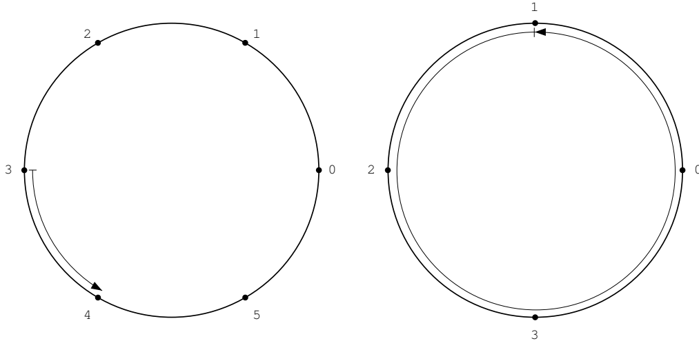
FIGURE 3. f \in \text{Hom}(\Lambda_5, \Lambda_3) , \tilde{f}(j) = 1 \quad \forall j \in \mathbb{Z}/6\mathbb{Z} , f is constant on [4, 3] and equal to 1; it makes a complete turn on [3, 4]
