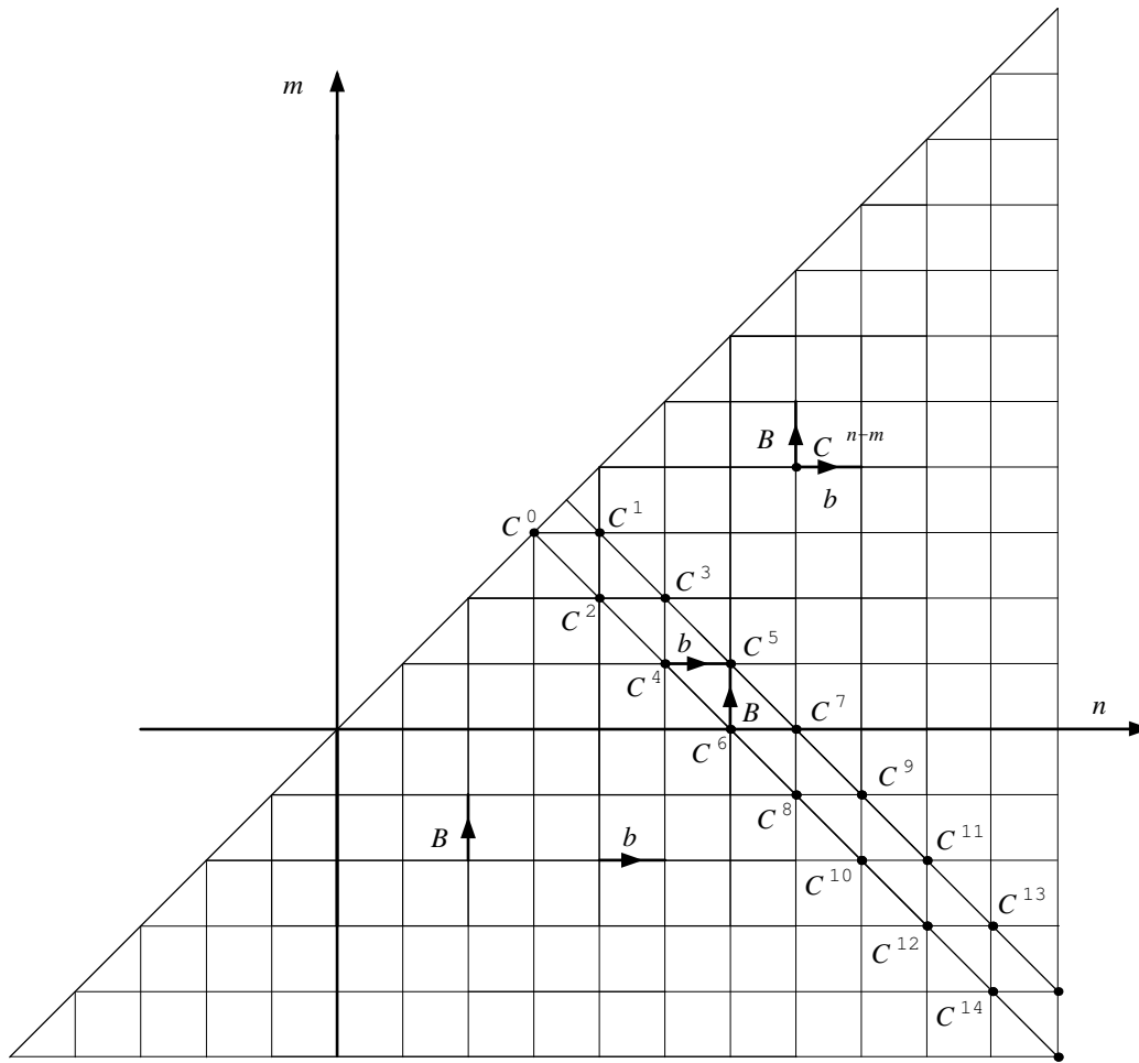
FIGURE 9. Bicomplex
