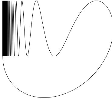
FIGURE 9. A compact space X with \pi_1(X) = \{0\} .
