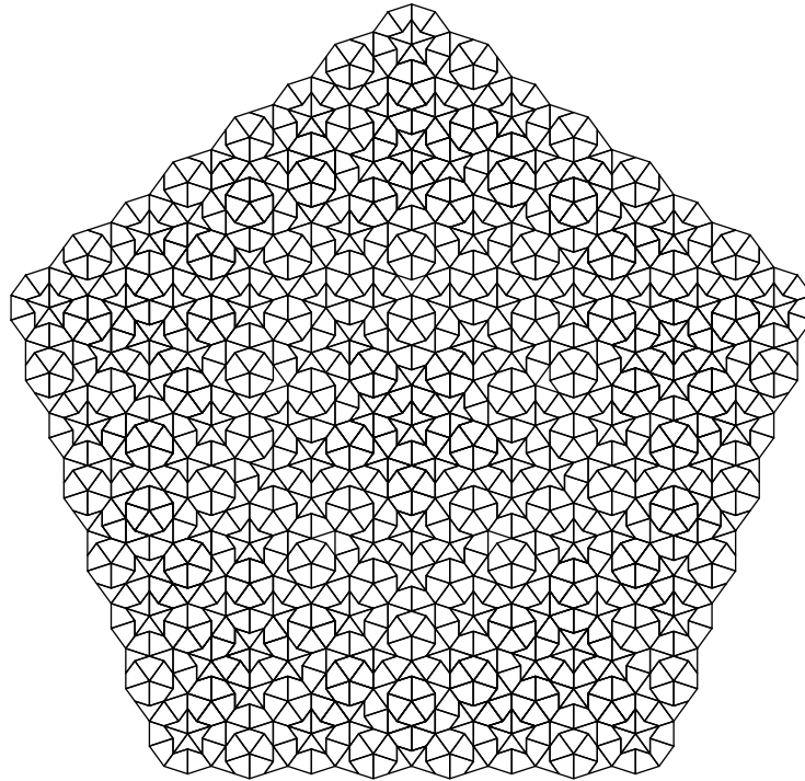
FIGURE 3. Penrose tiling
