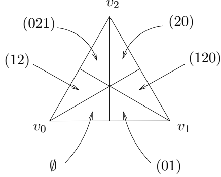
Figure 9: sd(\Delta^2)
