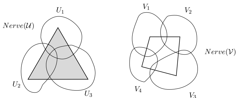
Figure 13: The nerves of two open covers
