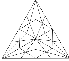
Figure 10: sd^2(\Delta^2)
