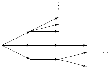
FIGURE 9.1. Non-empty tree.
