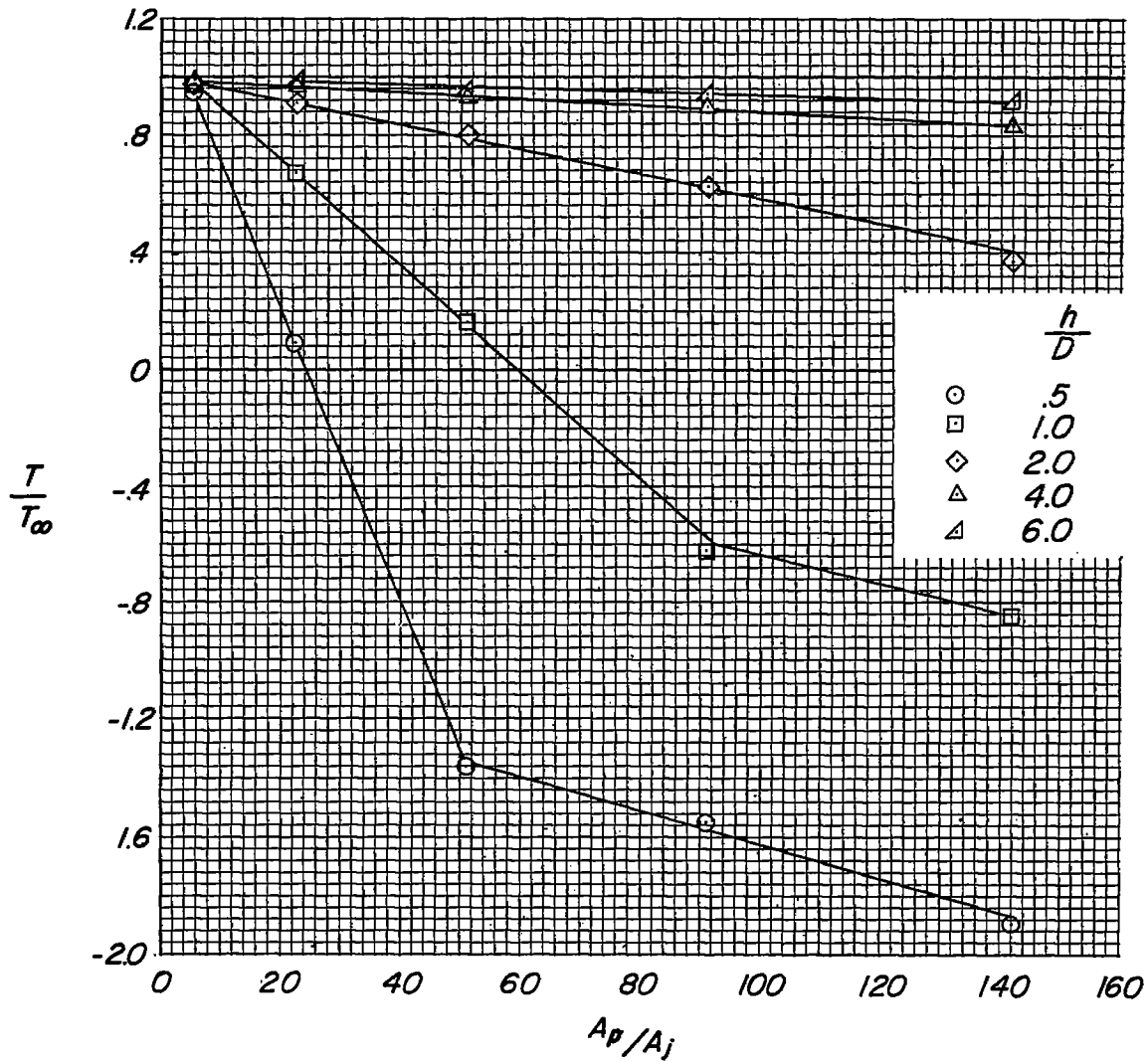
Figure 20.- Variation of T/T_\infty with ratio of area of square plates to area of jet at different heights above ground. \frac{P_{p,\infty}}{P} = 2.12 ; x/D = 0 .
