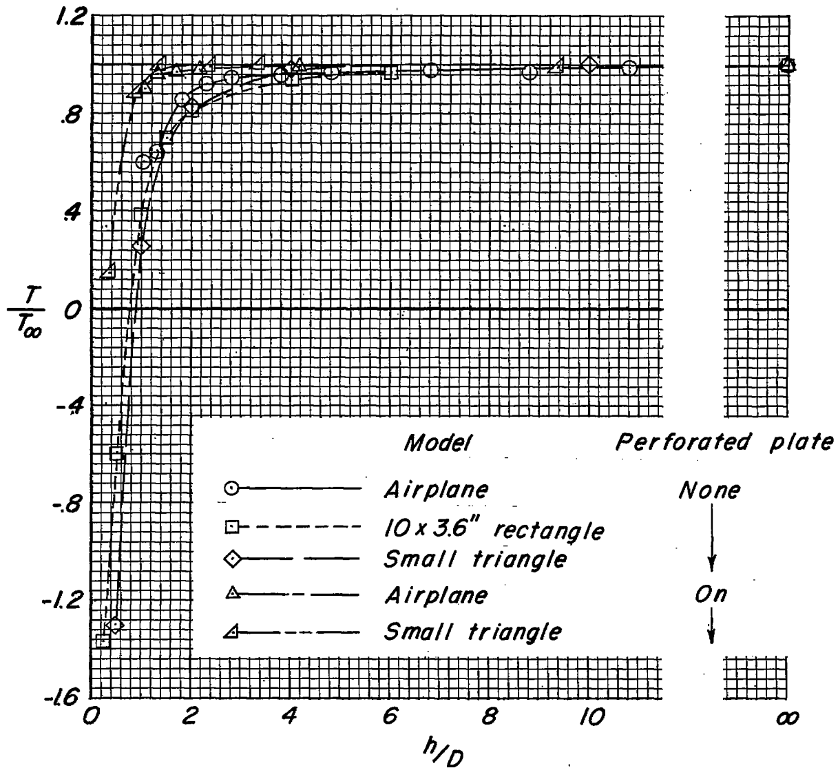
Figure 17.- Effect of plan form and perforated plate on T/T_{\infty} . Perforated plate 1/2 inch above ground when installed; \frac{P}{P_{\infty}} = 2.12 . (Note that area of each model equals approximately 36 square inches; x/D = 0 .)
