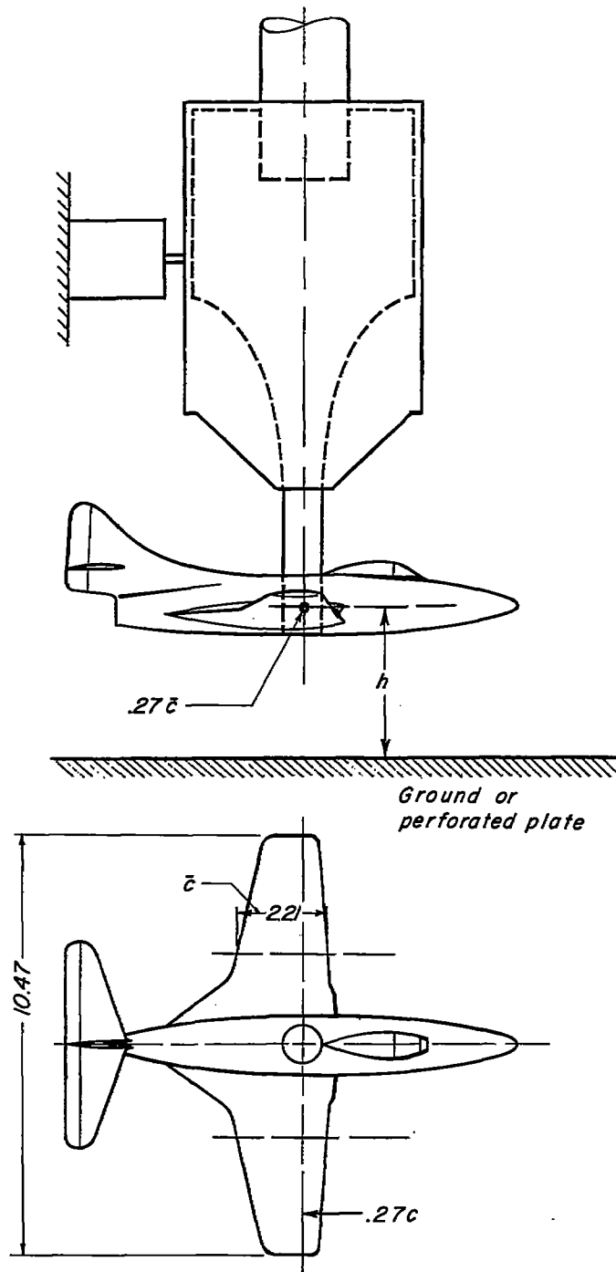
Figure 4.- Fighter-airplane-model installation. All dimensions are in inches.
