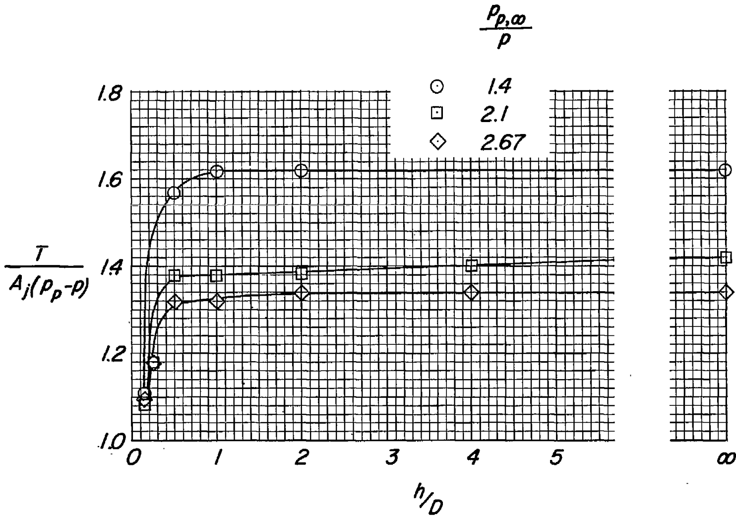
Figure 9.- Effect of ground proximity on thrust of nozzle nondimensionalized with respect to jet area and gage pressure.
