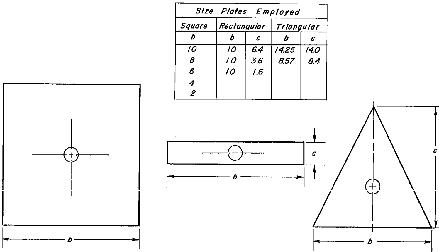
Figure 2.- Size and shape of different flat plates tested. All dimensions are in inches. (Plates are 1/8 inch thick.)
