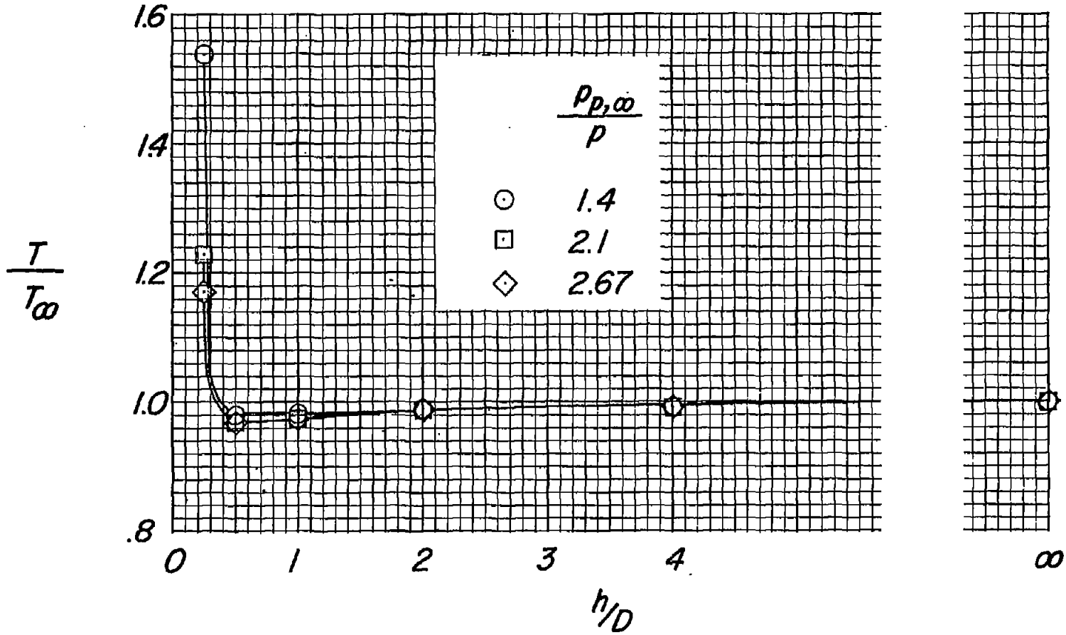
Figure 8.- Effect of ground proximity on thrust of nozzle alone for three plenum-chamber pressure ratios employed.
