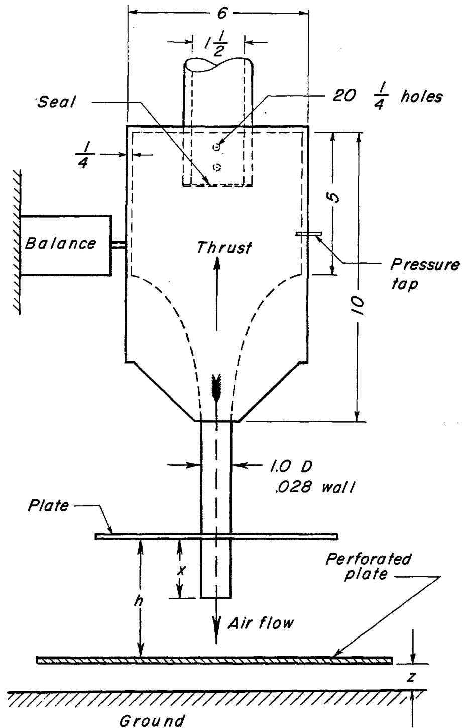
Figure 1.- Sketch of setup for nozzle, plates, and ground board. All dimensions are in inches.
