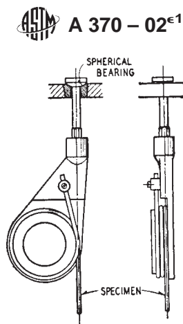
FIG. A4.2 Snubbing-Type Gripping Device
