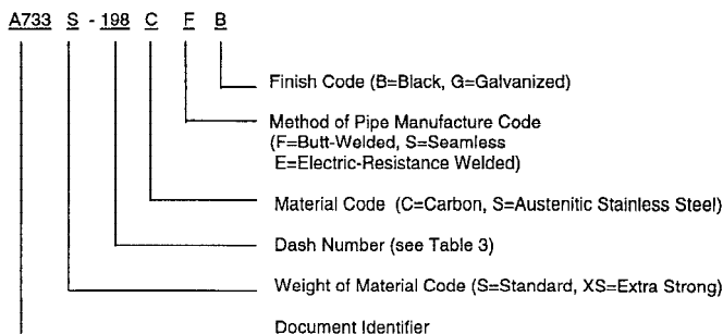
FIG. S1 Construction of Part Identifying Number
