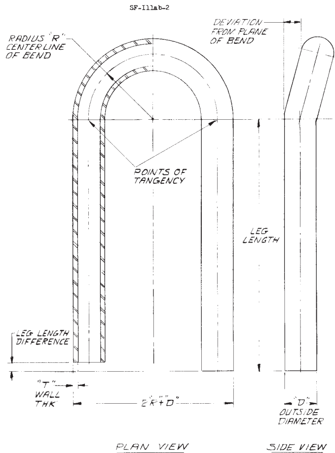
FIG. 1 Plane Bend for U-Tube
