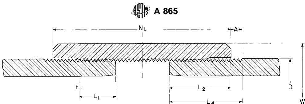
FIG. 3 Recessed Taper-Tapped Coupling and Pipe (See Table 4 for Coupling Dimensions)
