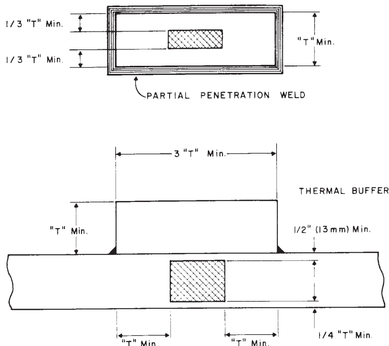
NOTE 1—Longitudinal axis and gage length of test specimen must be within cross-hatched zone. FIG. S26.4 Thermal Buffer Pads
