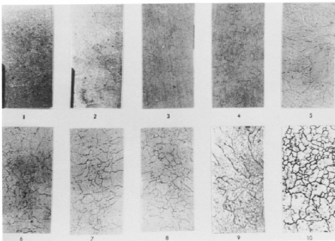
NOTE 1—The 10 levels of severity of intergranular network structures shown are indicative of the presence of aluminum nitride precipitation in the primary austenitic grain boundaries.
