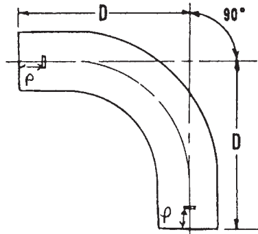
FIG. 7 Sixteenth Bends
