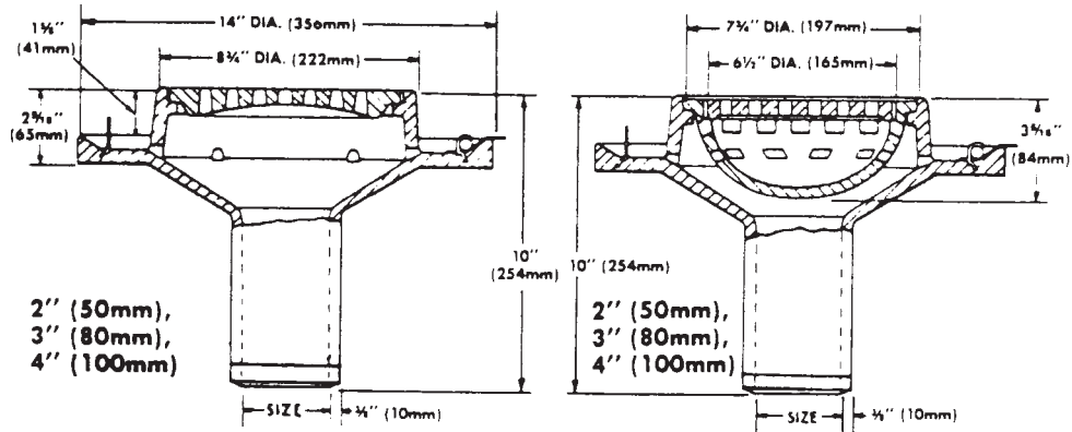
FIG. 34 Floor Drains
