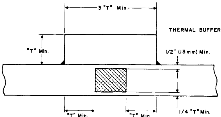
NOTE—Longitudinal axis and gage length of test specimen must be within cross-hatched zone. FIG. S26.4 Thermal Buffer Pads
