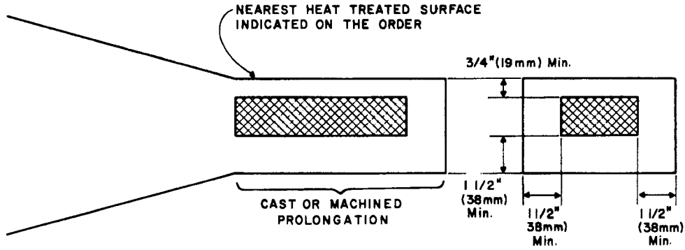
FIG. S26.2 Prolongation Test Specimen
