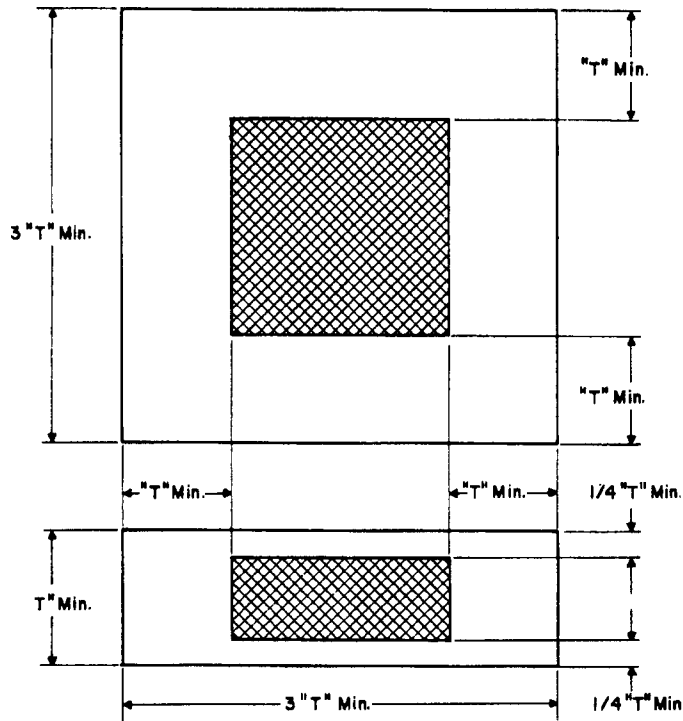
FIG. S26.3 Separately Cast Block
