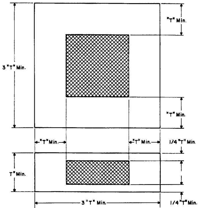
FIG. S26.2 Prolongation Test Specimen
