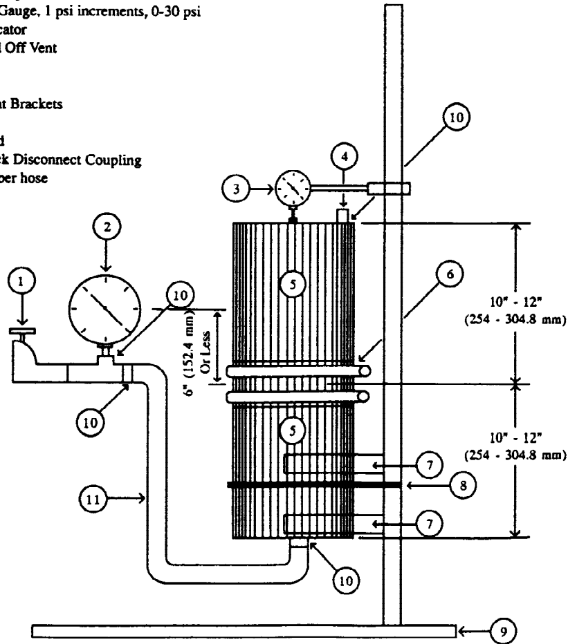
FIG. 3 UNRESTRAINED restrained HYDROSTATIC hydrostatic JOINT Joint T-TEST
