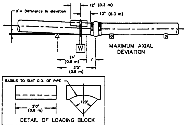
FIG. 1 Deflection Test (Plan View)
