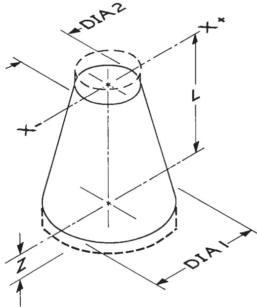
NOTE 1—Top or bottom, or both, of this shape may be slanted. FIG. 23 Shape 5.1—Reducer-Round
