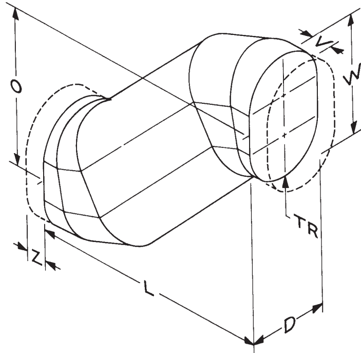
FIG. 5 Shape 2.2.1—Offset-Flat Oval-Long Axis
