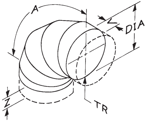
FIG. 13 Shape 3.1—Elbow-Round
