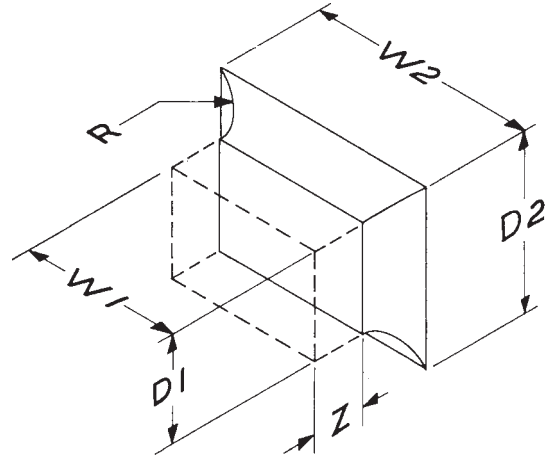
FIG. 32 Shape 6.6.2—Bellmouth-Rectangular
