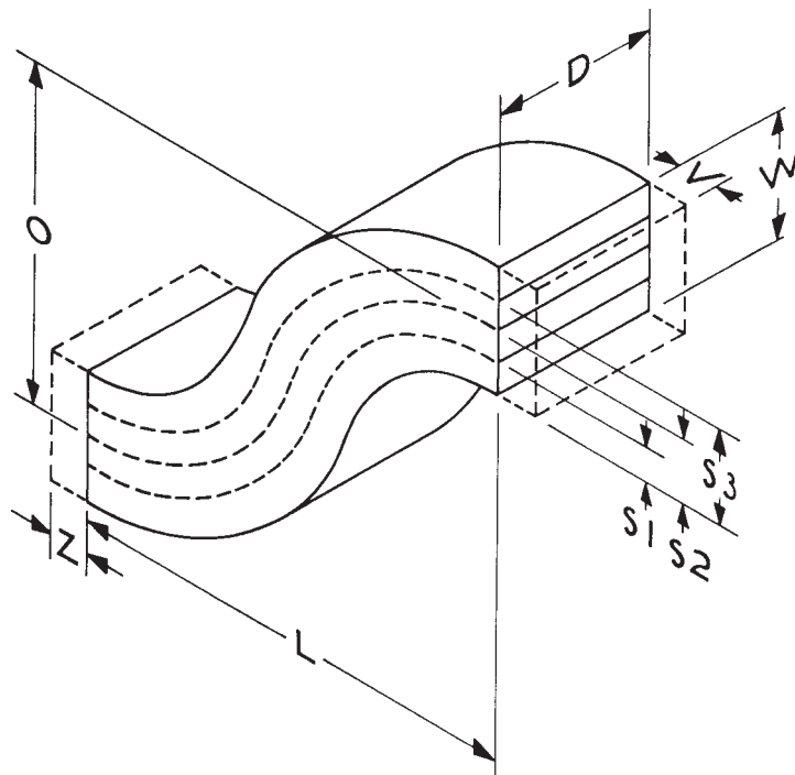
FIG. 10 Shape 2.4.2—Offset-Ogee With Splitters
