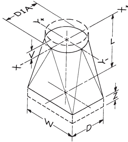
FIG. 27 Shape 6.2—Transition-Rectangular to Round
