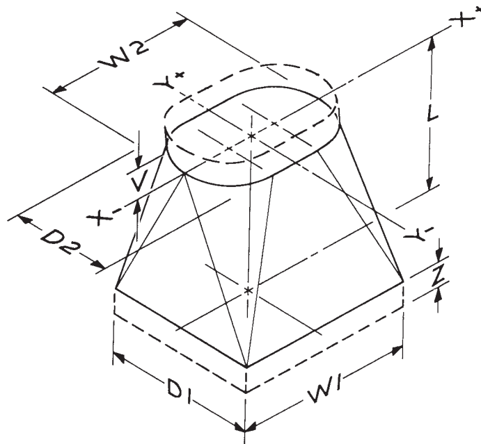
FIG. 28 Shape 6.3—Transition-Rectangular to Flat Oval
