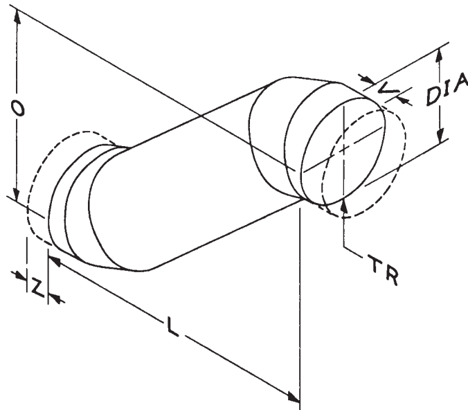
FIG. 4 Shape 2.1—Offset-Round
