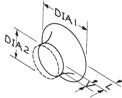
FIG. 31 Shape 6.6.1—Bellmouth-Round
