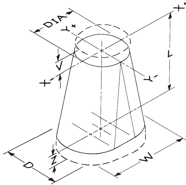
NOTE 1—Top or bottom, or both, of this shape may be slanted. FIG. 26 Shape 6.1—Transition-Flat Oval to Round
