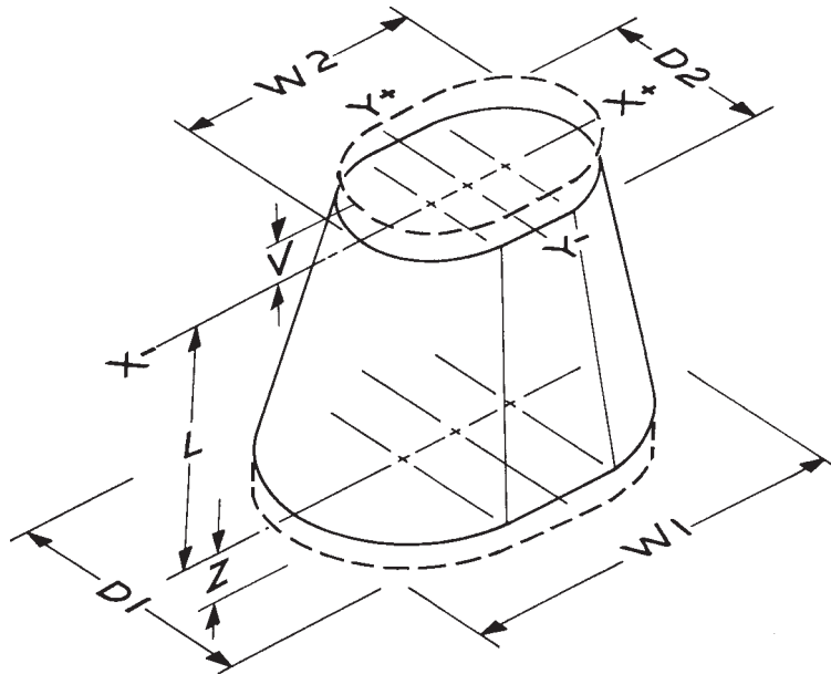
NOTE 1—Top or bottom, or both, of this shape may be slanted. FIG. 24 Shape 5.2—Reducer-Flat Oval
