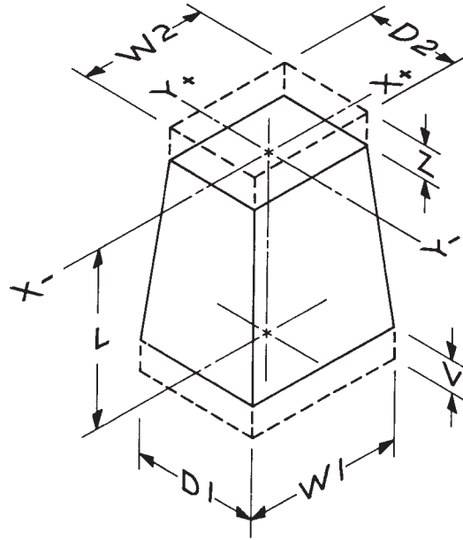
NOTE 1—Top or bottom, or both, of this shape may be slanted. FIG. 25 Shape 5.3—Reducer-Rectangular
