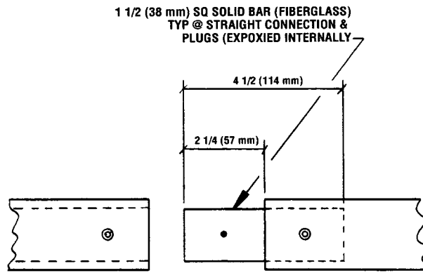
FIG. 8 Splice
