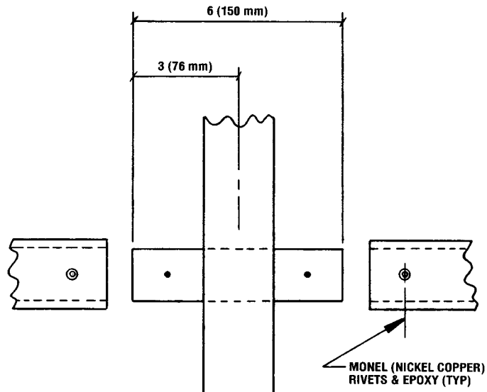
FIG. 9 Midrail to Stanchion
