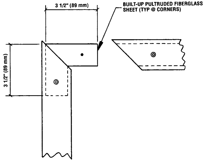
FIG. 7 Corner Connection
