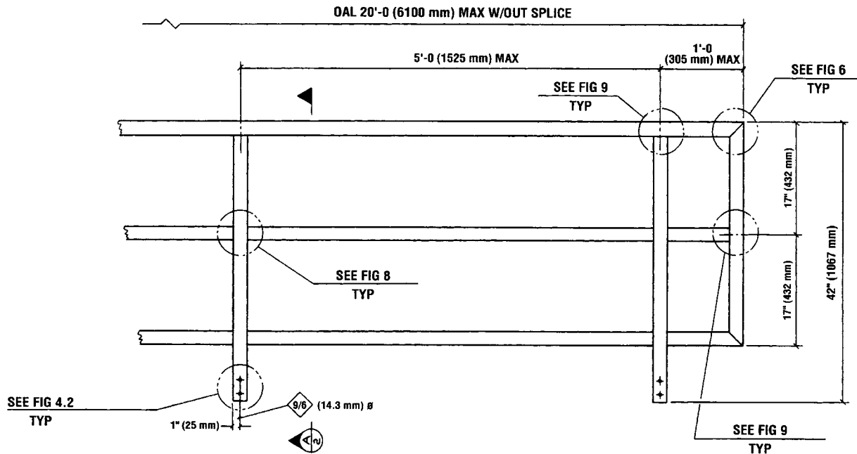
FIG. 6 Three-Course Rail
