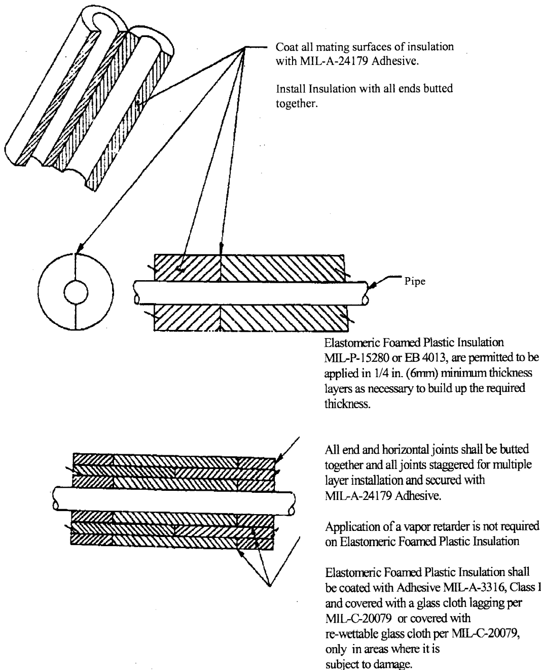
FIG. 2 Installation of Elastomeric Foamed Plastic Insulation (MIL-P-15280 or EB 4013)
