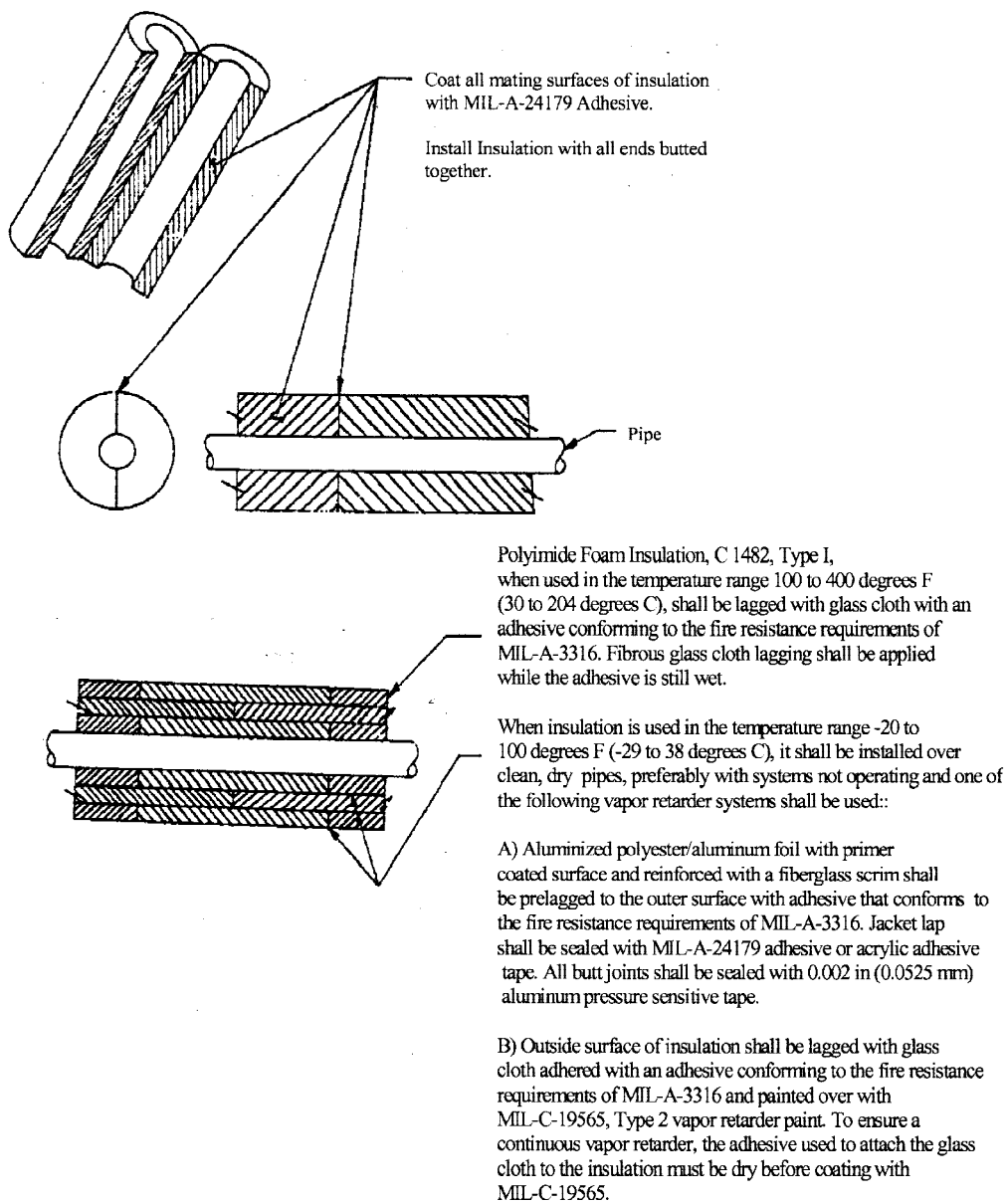
FIG. 3 Installation of Polyimide Foam Insulation (Specification C 1482)
