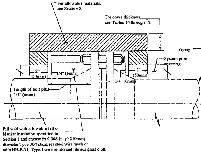
FIG. 16 Typical Removable Flange Cover Where Flange Diameter is Larger Than the Outside Diameter of the Adjacent Pipe Covering
