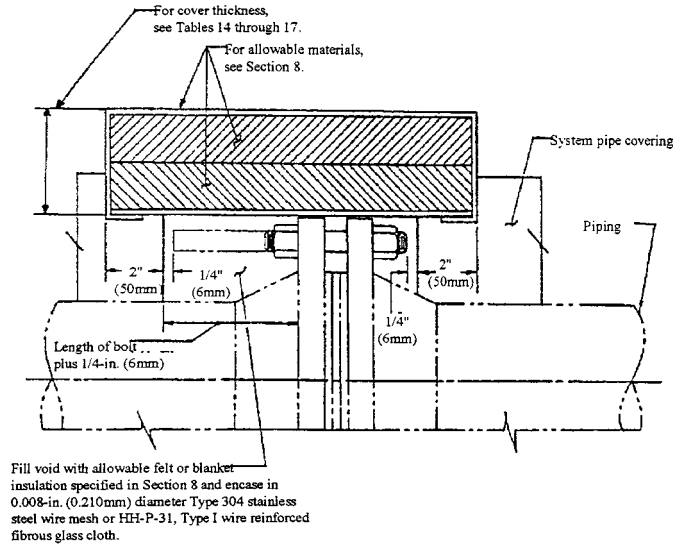
FIG. 17 Typical Removable Flange Cover Where Flange Diameter is Smaller Than the Outside Diameter of the Adjacent Pipe Covering
