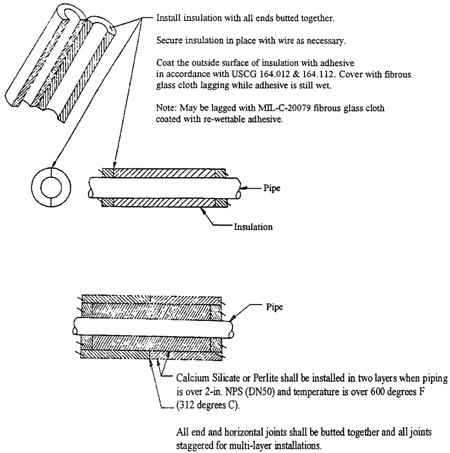
FIG. 5 Installation of Calcium Silicate Pipe Insulation (Specification C 533) and Perlite Pipe Insulation (Specification C 610)
