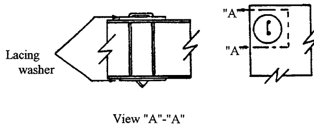
Using Lacing Washers FIG. 23 Typical Methods of Quilting Removable Covers
