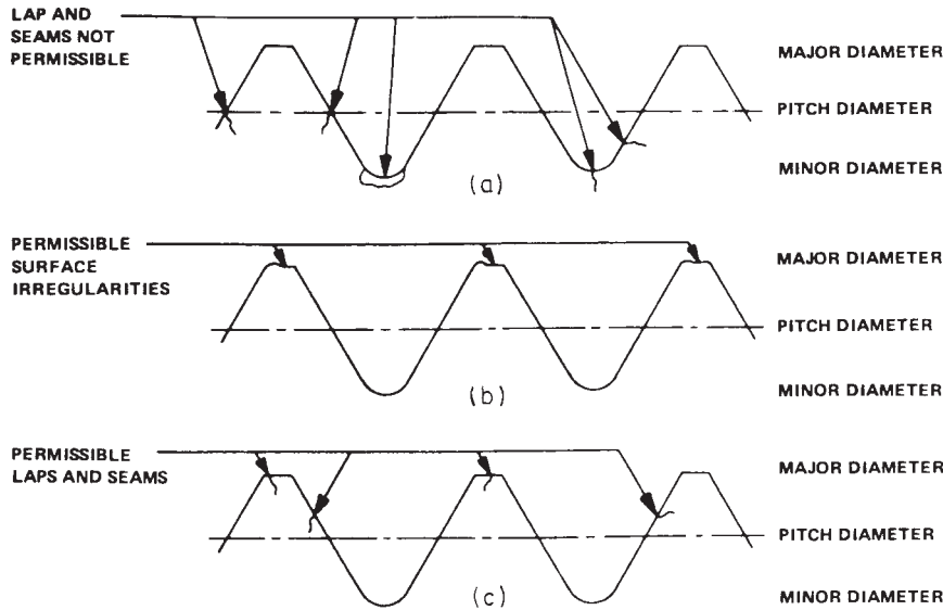
FIG. 4 Thread Discontinuities
