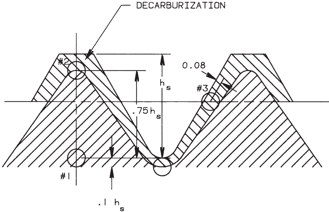
FIG. 1 Decarburization Limits
