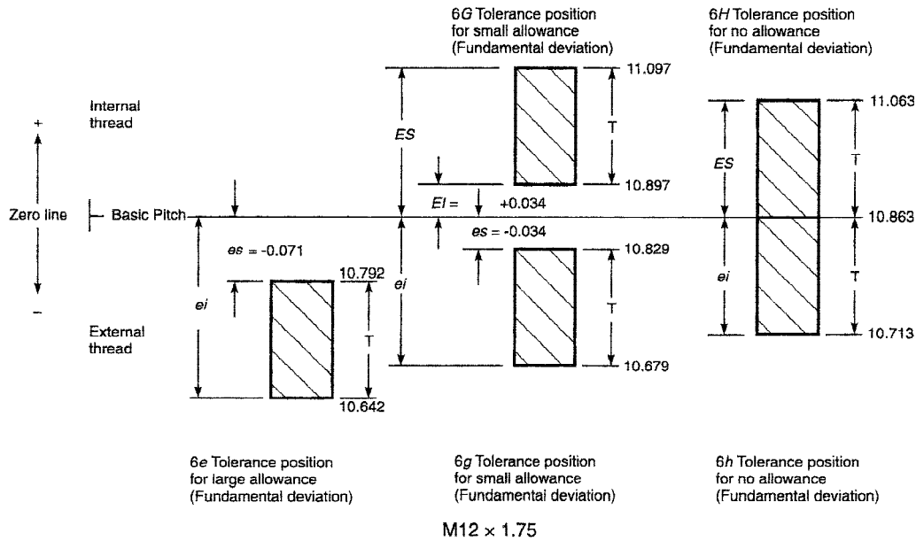
FIG. X3.1 Metric Tolerance System for Screw Threads
