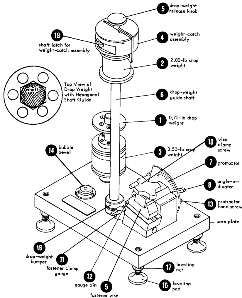
NOTE—This device is available from The National Wooden Pallet and Container Assn., 1625 Massachusetts Ave., Washington, DC 20036 FIG. 1 A Typical Impact Bend Tester for the Impact Bend Testing of Nails
