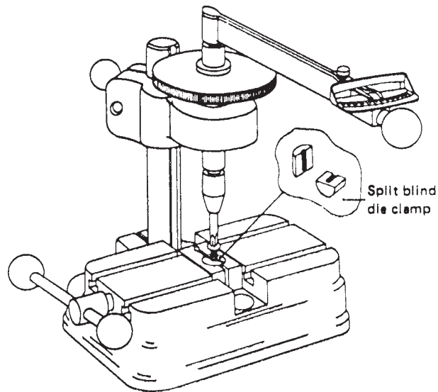
FIG. 2 Torque-Measuring Device
