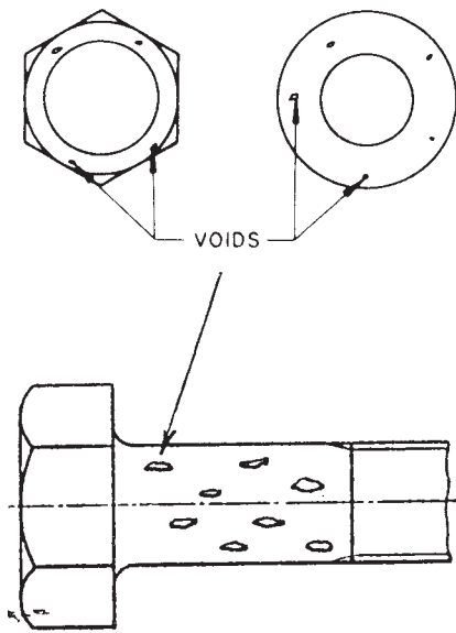
FIG. 6 Typical Voids
