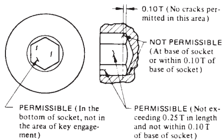
FIG. 3 Socket Discontinuity Limitations
