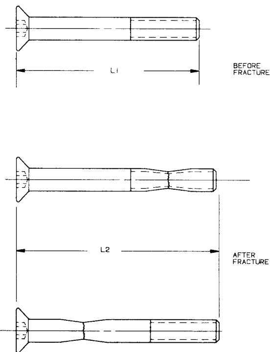
FIG. 4 Test Specimen-Extension Test
