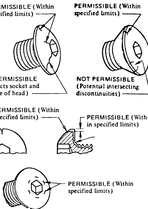
FIG. 1 Head Discontinuities (See 10.2.1)
