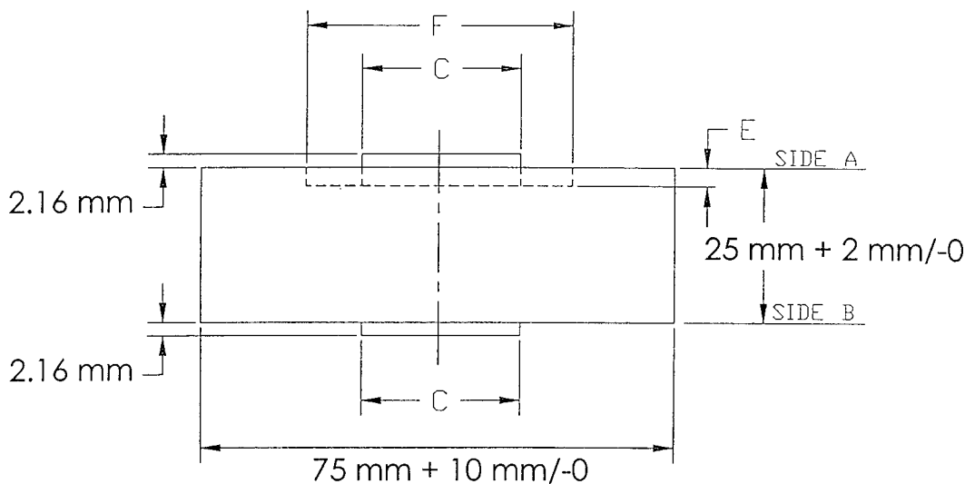
FIG. A1.1 Support Block
