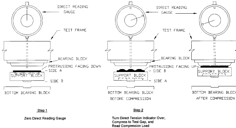
FIG. A1.3 Steps for Determining Compression Load
