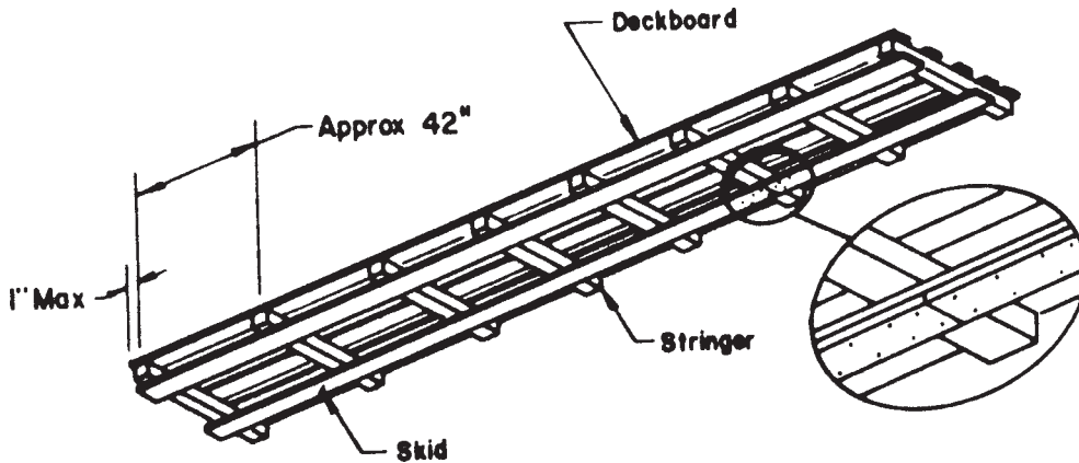
FIG. 17 Double Faced Pallet with Laminated Skids (Runners) D
