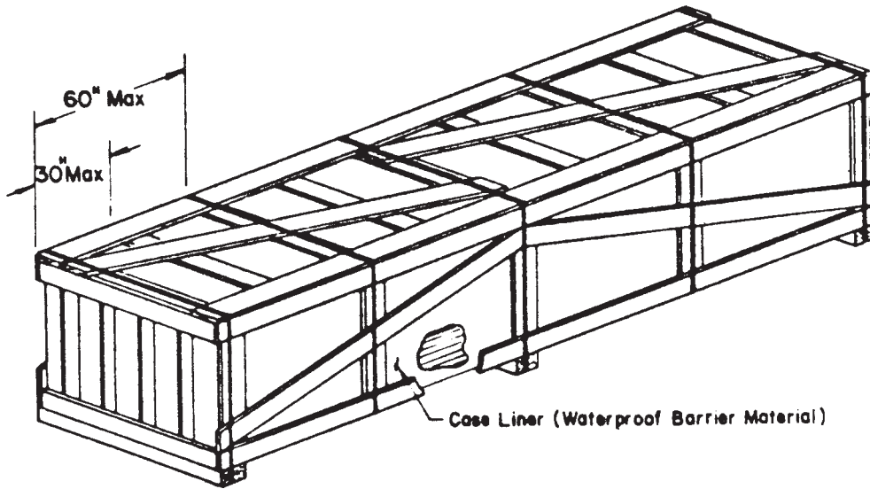
FIG. 23 Style 3 Crate, Open G G For pipe.
