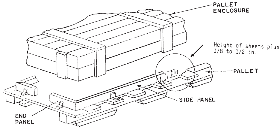
FIG. 21 Pallet Enclosure J
