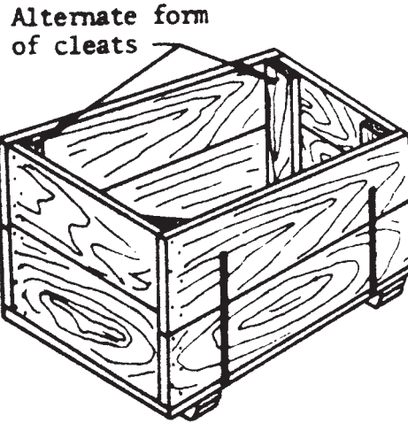
FIG. 5 Style 5 Nail Wood Box A
