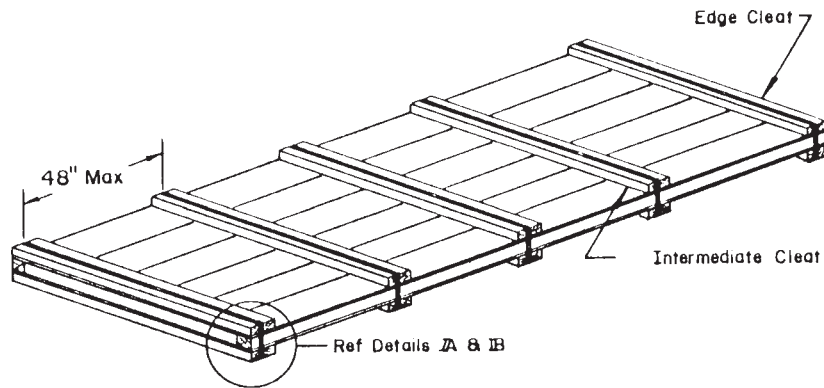
FIG. 23 Style 3 Crate, Open G G For pipe.
