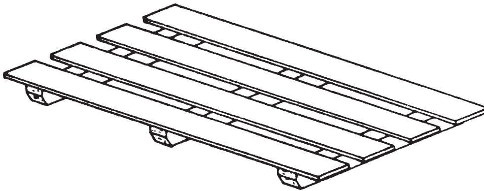
FIG. 16 Pallet with Crosswise Skids. (Runners) C
