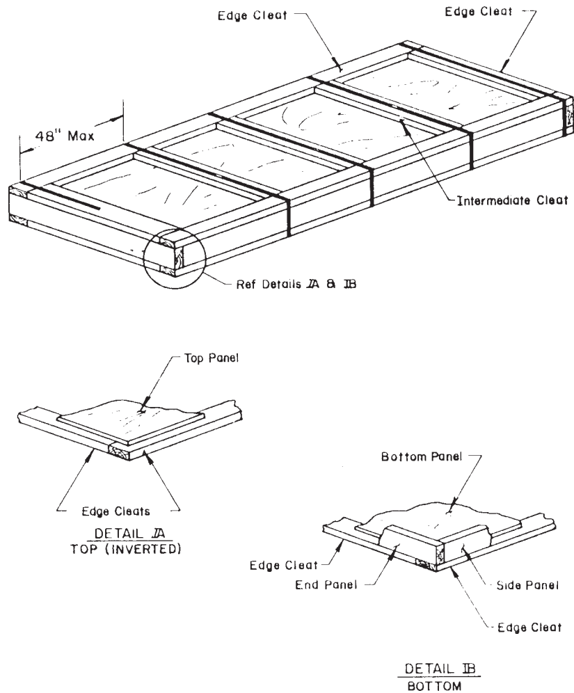
FIG. 25 Plywood or Paper Overlaid Veneer Box (Telescopic) for Flat Sheet K
