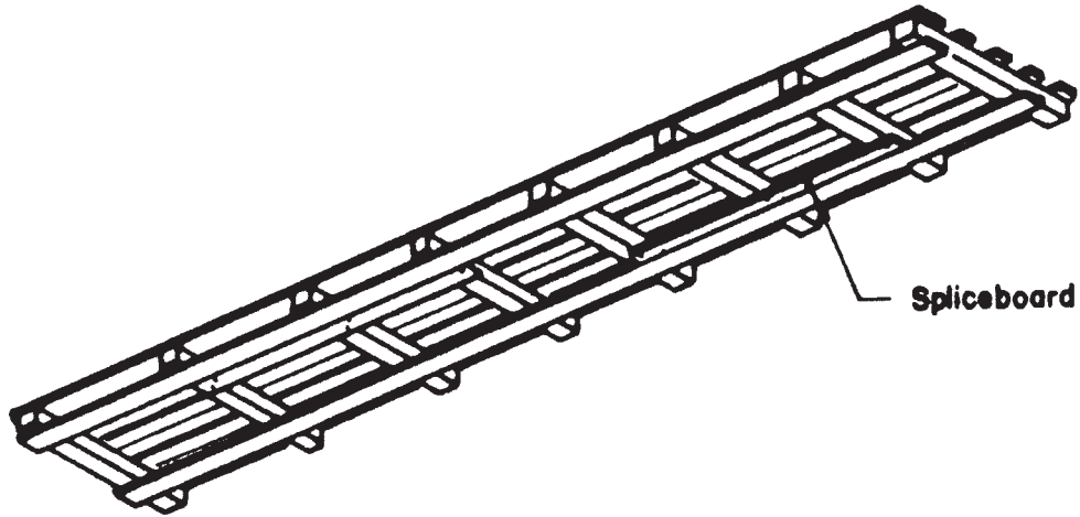
FIG. 18 Double Faced Pallet with Spliceboards D D For plate and plate circles; sheet, flat, or coiled roofing and siding.
