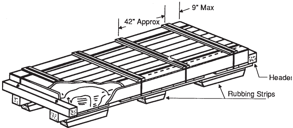
FIG. 19 Pallet Enclosure E (Headers mandatory for DoD, otherwise optional)
