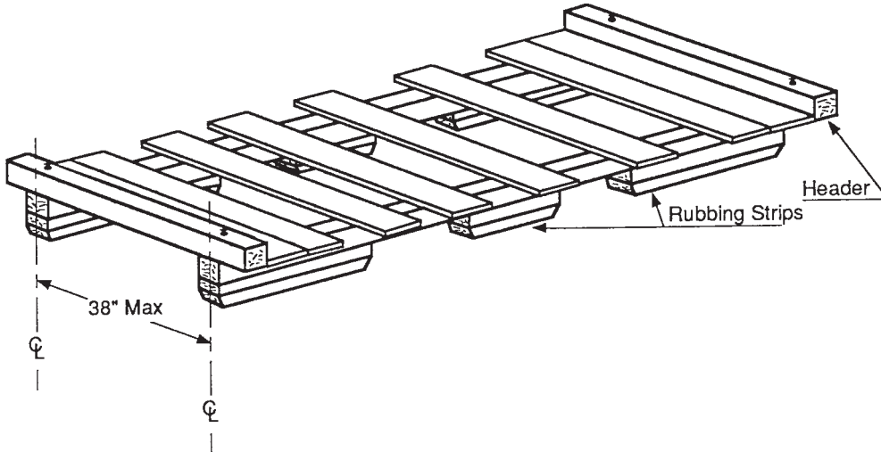
FIG. 15 Pallet with Lengthwise Skids (Runners) C (Headers mandatory for DoD, otherwise optional)
