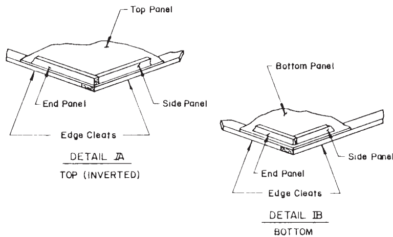
FIG. 26 Solid Fiberboard Panel Box (Telescopic) for Flat Sheet K
