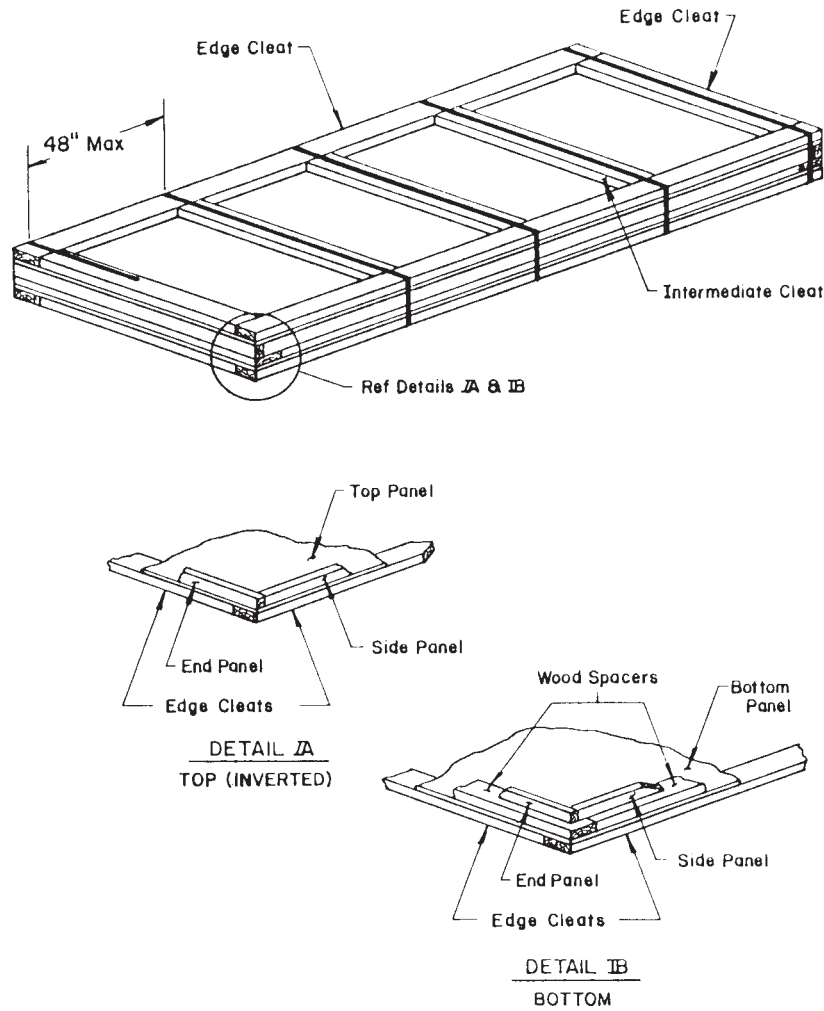
FIG. 27 Solid Fiberboard Panel Box, With Spacer (Telescopic) for Flat Sheet K
