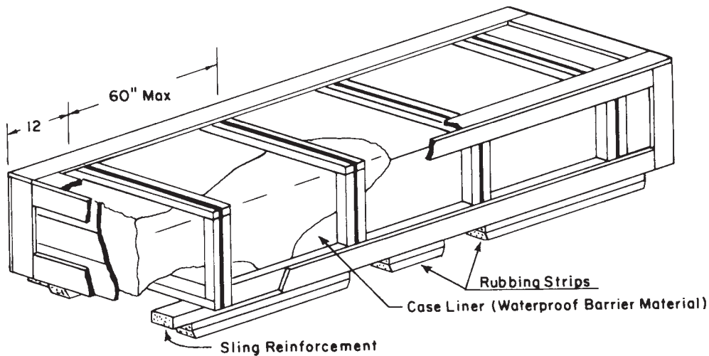
FIG. 22 Style 2 Crate, Open (Rubbing strips mandatory for DoD, otherwise optional) G
