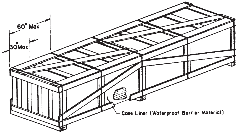
FIG. 273 Style 3 Crate, Open c c For pipe.
