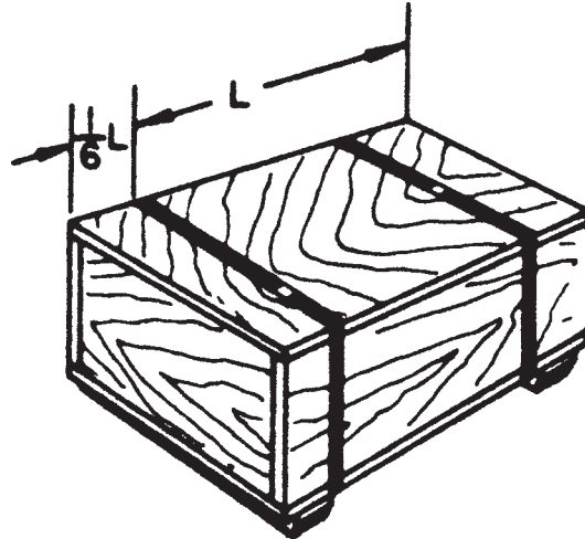
FIG. 6.2 Style 1 Nail Wood Box A
