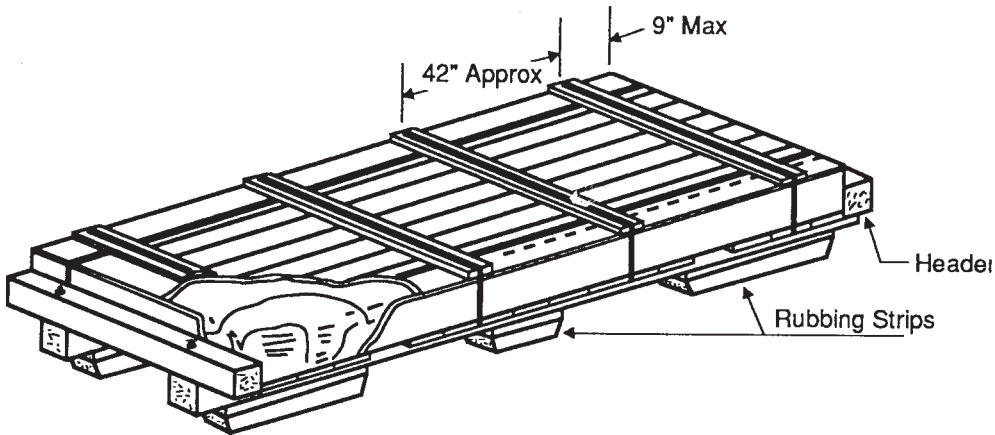
FIG. 23 19 Pallet Enclosure E (Headers mandatory for DoD, otherwise optional)
