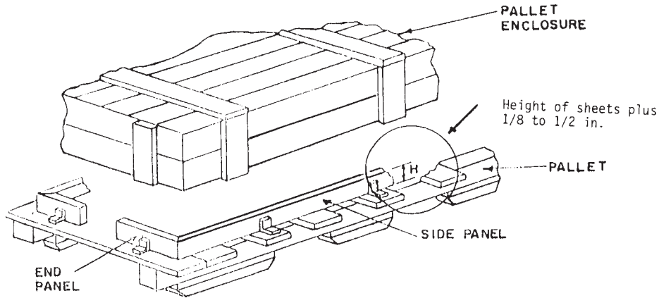
FIG. 251 Pallet Enclosure d
