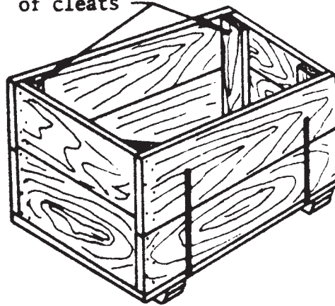
FIG. 9 5 Style 5 Nail Wood Box A
