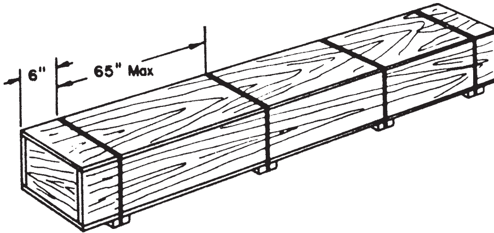
FIG. 10 6 Style 1 Nail Wood Box B
