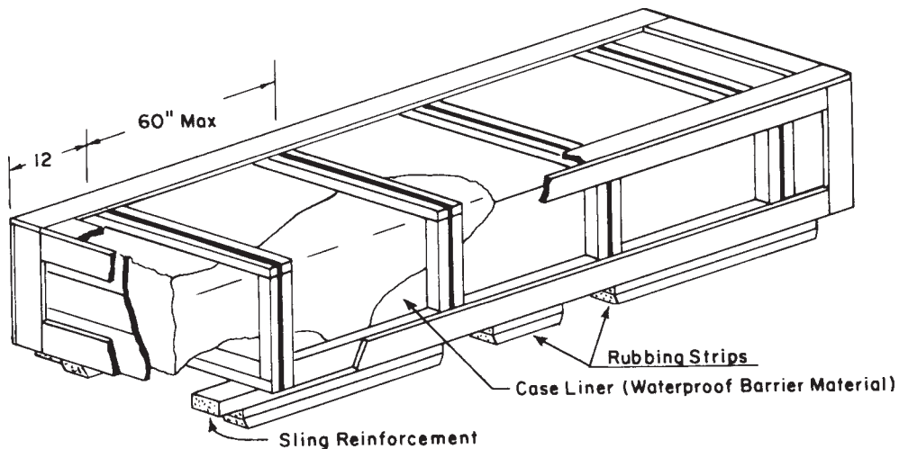
FIG. 262 Style 2 Crate, Open (Rubbing strips mandatory for DoD, otherwise optional) e
