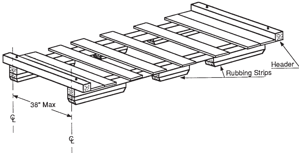
FIG. 195 Pallet with Lengthwise Skids (Runners) C (Headers mandatory for DoD, otherwise optional)
