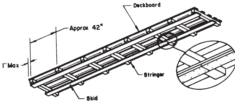
FIG. 2 17 Double Faced Pallet with Laminated Skids (Runners) D
