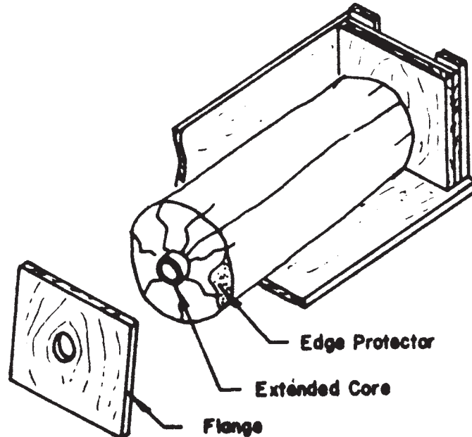
FIG. 162 Coil Foil Packing (See 7.9)
