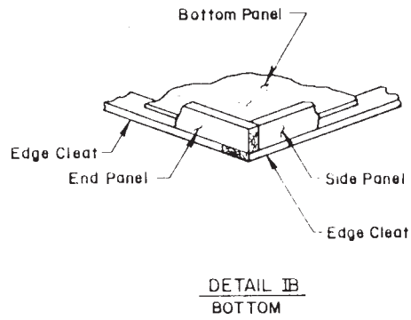
FIG. 25 Plywood or Paper Overlaid Veneer Box (Telescopic) for Flat Sheet K
