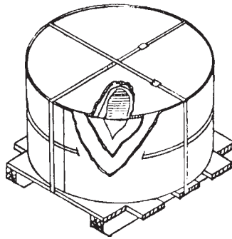
FIG. 33 Fiber Enclosed Skid for Coil
