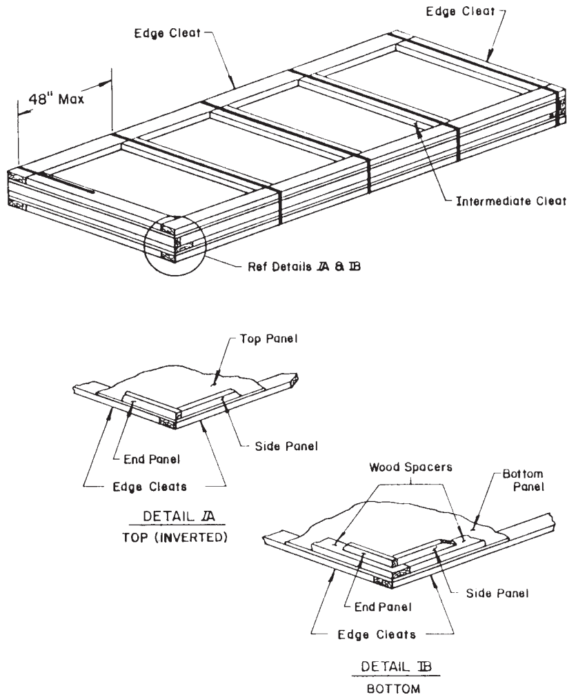
FIG. 4 27 Solid Fiberboard Panel Box, With Spacer (Telescopic) for Flat Sheet K
