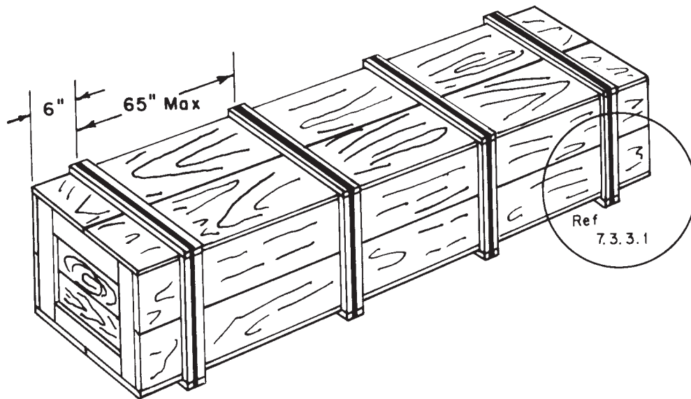
FIG. 12 8 Style 2 Nail Wood Box B
