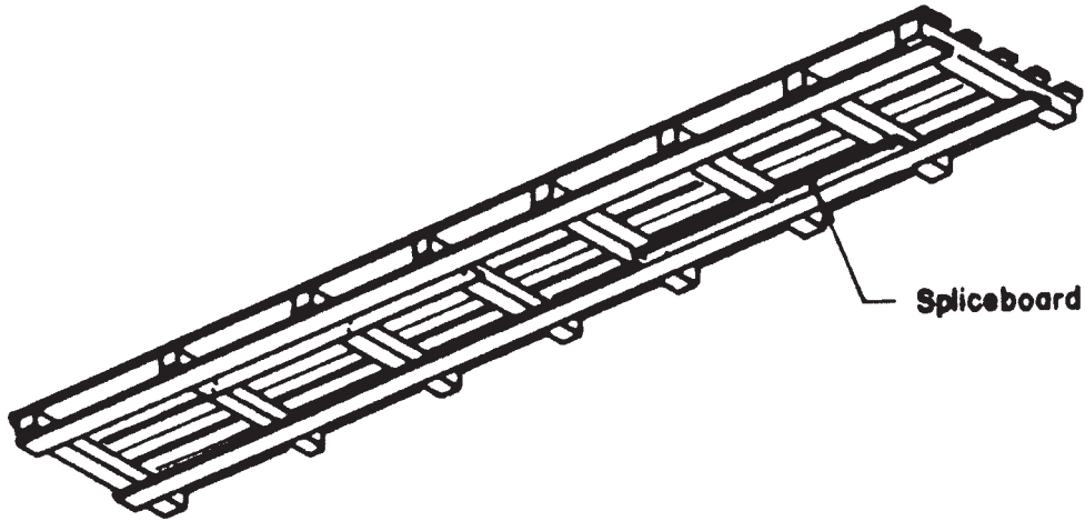
FIG. 22 18 Double Faced Pallet with Spliceboards D D For plate and plate circles; sheet, flat, or coiled roofing and siding.
