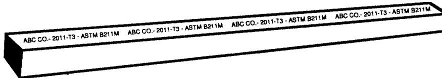
FIG 4 Continuous Marking for Rod, Bar, Profiles and Tube in Straight Lengths
