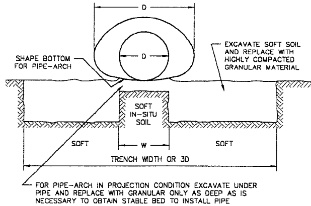
FIG. 4 Soft Foundation Treatment
