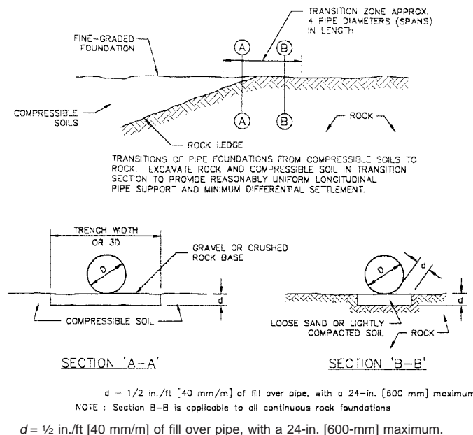
FIG. 3 Foundation Transition Zones and Rock Foundations
