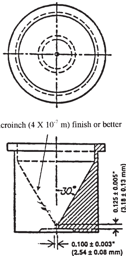
FIG. 1 Flowmeter Funnel
