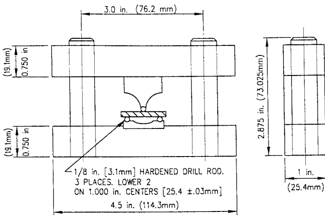
FIG. 3 Transverse Rupture Test Fixture
