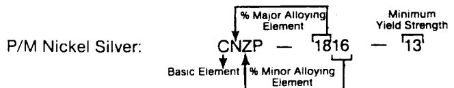
FIG. X1.1 Illustration of Powder Metallurgy Nonferrous Material Designation Coding
