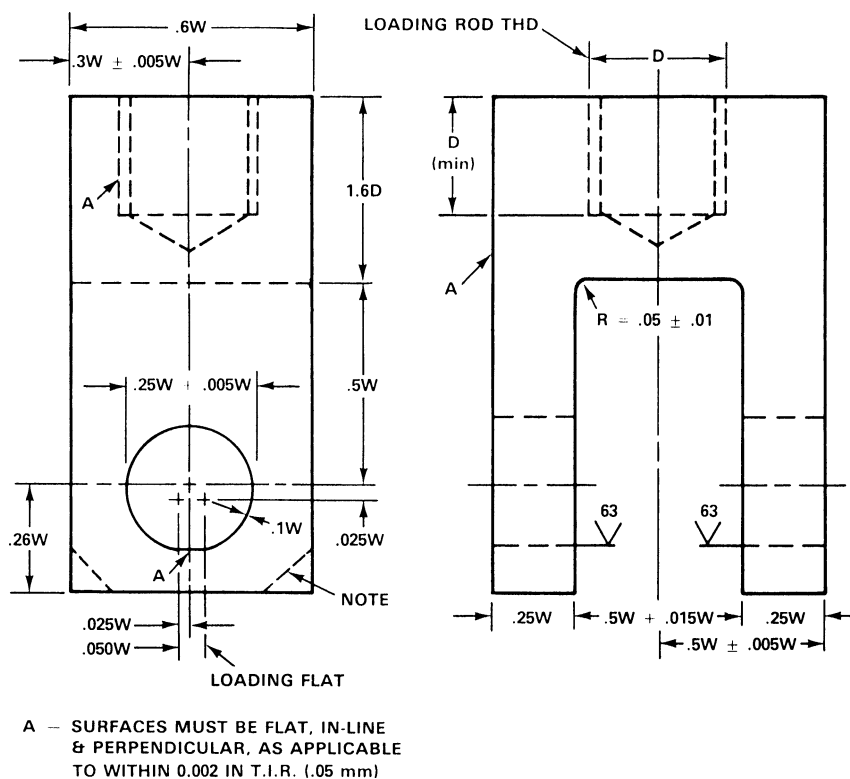
FIG. 3 Clevis for C(T) Specimen Testing
