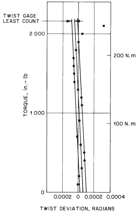
FIG. 2 Torque-Deviation Graph
