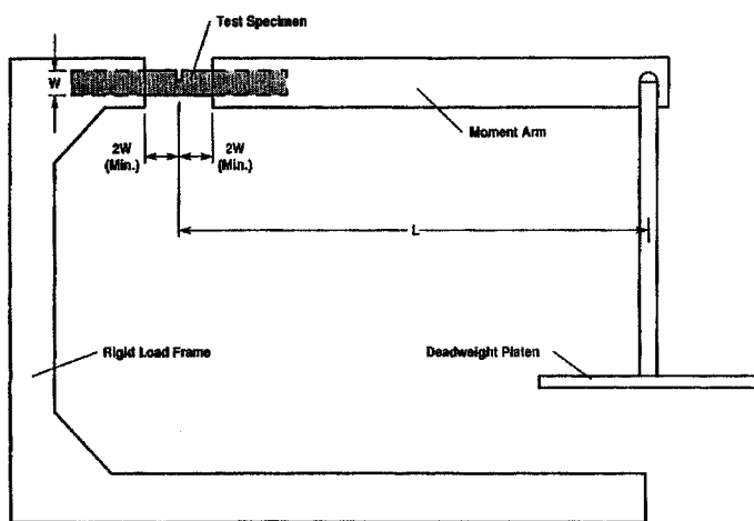
NOTE 1—The length of the moment arm (L) should be equal to or greater than 8W
