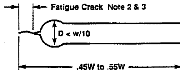
Slot Ending in Drilled Hole
