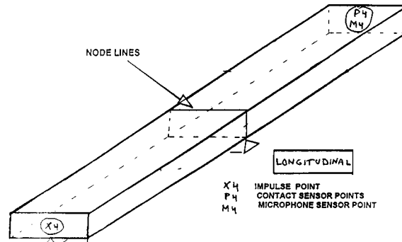
FIG. 7 Rectangular Specimen Tested for Longitudinal Vibration
