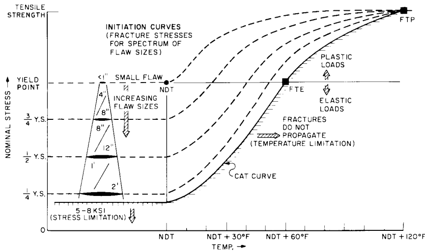
FIG. 1 Generalized Fracture Analysis Diagram Indicating the Approximate Range of Flaw Sizes Required for Fracture Initiation at Various Levels of Nominal Stress, as Referenced by the NDT Temperature 1
