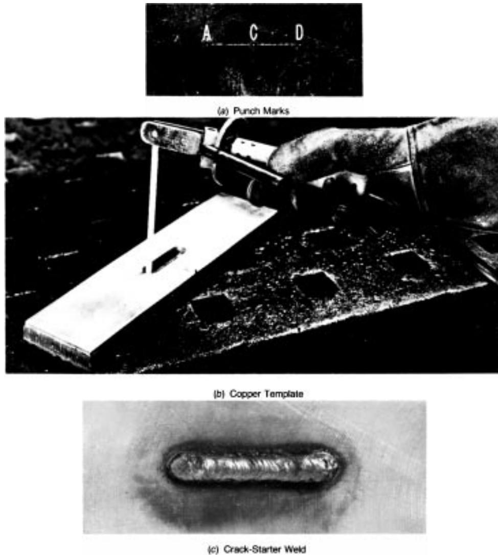
FIG. 7 Methods of Locating the Weld Deposit Properly on the Test Specimen
