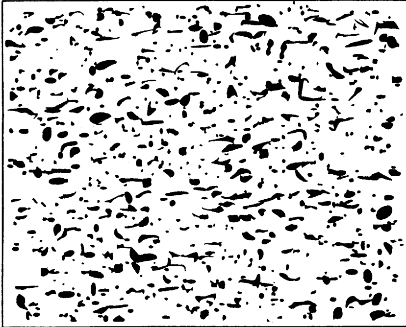
FIG. 7 — 15.0 % Porosity
