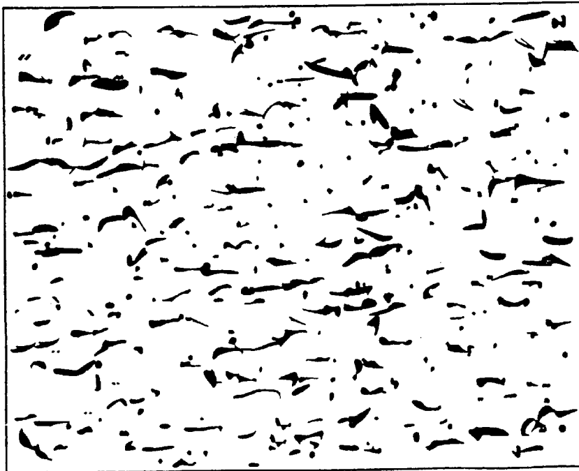
FIG. 6 — 10.0 % Porosity
