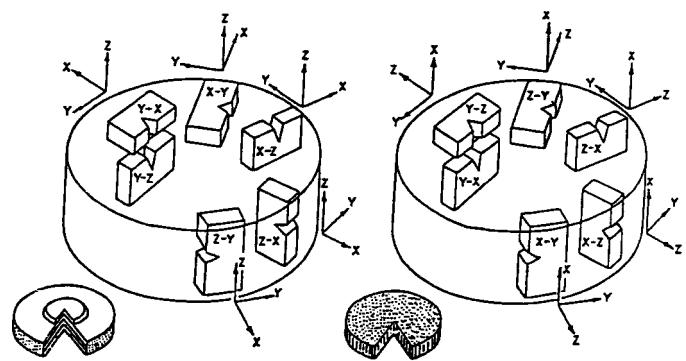
a) Radial grain flow, axial working direction b) Axial grain flow, radial working direction
