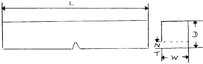
FIG. A4.2 Charpy (Simple-Beam, type A) Impact Test Specimen
