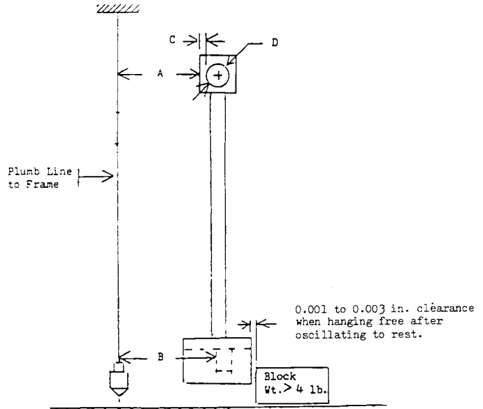
FIG. X2.1 Measurement of Deviation of Center of Strike from Vertical Plane through Axis of Rotation when Pendulum is Hanging Free
